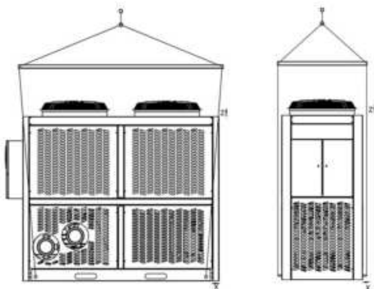
Figure 2. Recommended heat pump rigging
