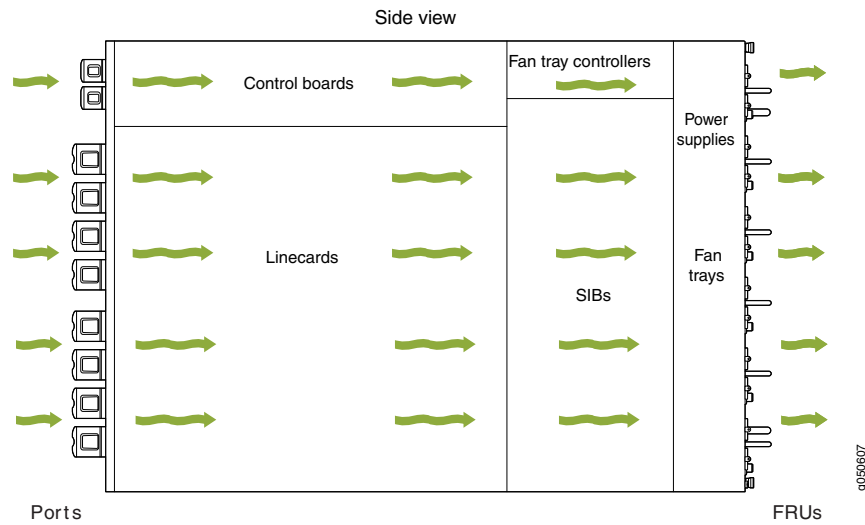
Figure 3: Top View of Airflow Through a PTX10008
