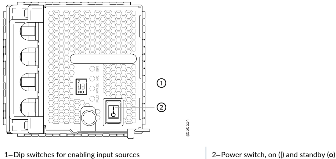
Figure 32: Setting the Enable Switches for the Power Source
