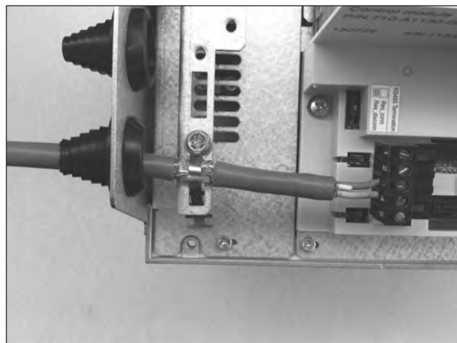
Figure 6. Control cable grounding
