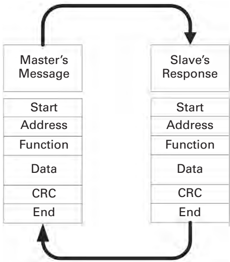
Figure 12. The basic structure of a modbus frame
