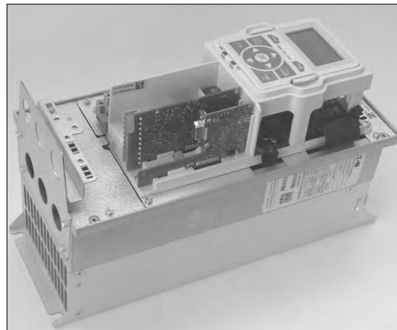
Figure 4. PowerXL Series control board location
