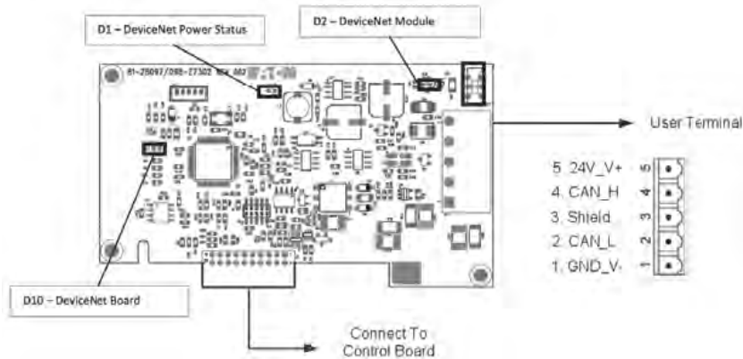
Figure 51. DeviceNet hardware
