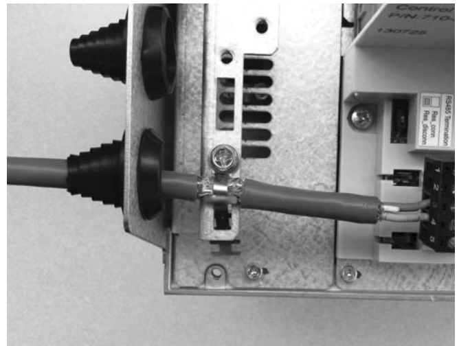
Figure 32. Serial ground
