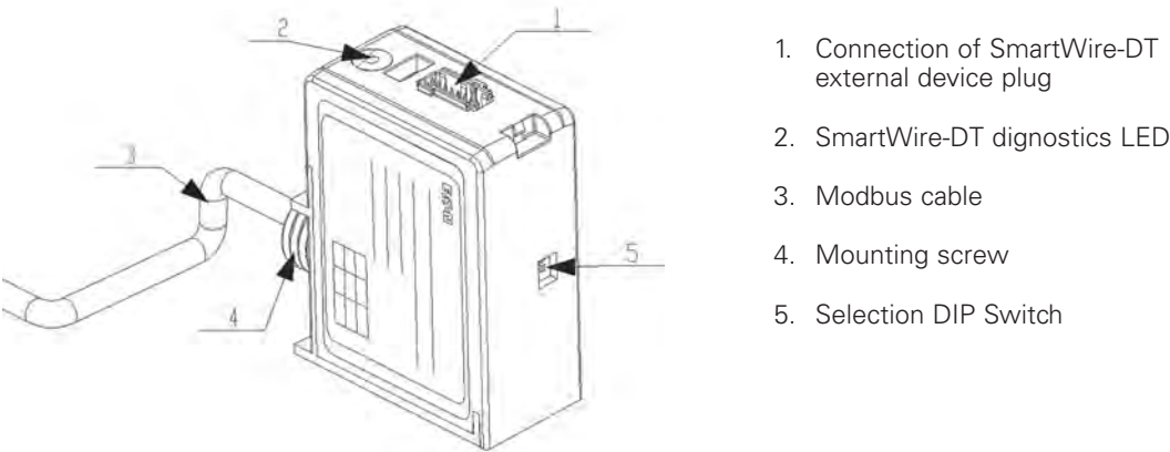
Figure 55. SmartWire-DT “DXG-NET-SWD-IP20” module details
