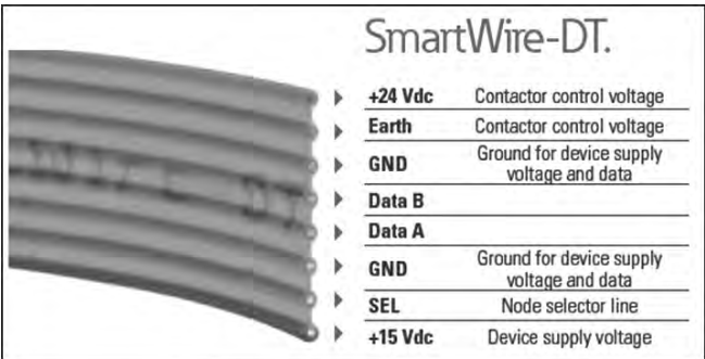
Figure 58. 5 core round cable and pin assignment SACC-E-MS-5CON-M16/0,5 SCO - 1520055
