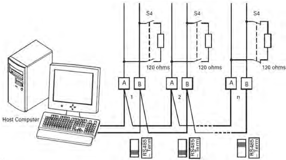
Figure 7. Connection diagram
