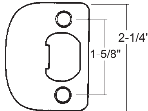
KW-83796 US-3, 5, 10B, 15, 26D 1/4" Radius Strike (RCS-4)
