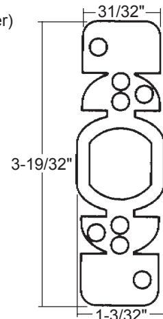
KW-81640 Strike Box Plastic door jamb deadbolt strike insert for cleaner installation
