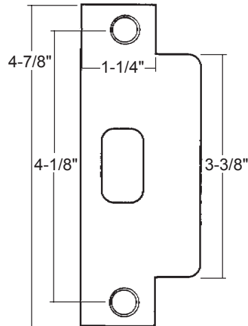
KW-83437 US-3, 5, 10B, 15, 15A Standard Lockset Strike
