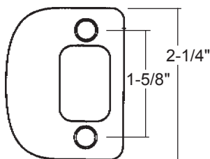
KW-85303 US-10B, 15 Deadbolt strike with lip. 1/4" radius corners.
