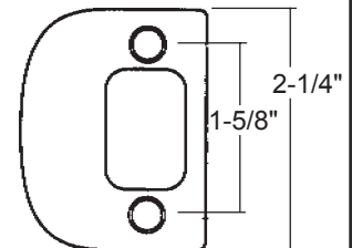
KW-84638 US-3, 26D Deadbolt strike with lip
