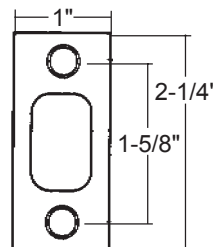
KW-85072 US-3, 15, 15A, 26D 660 Series Deadlock Strike Square corner strike
