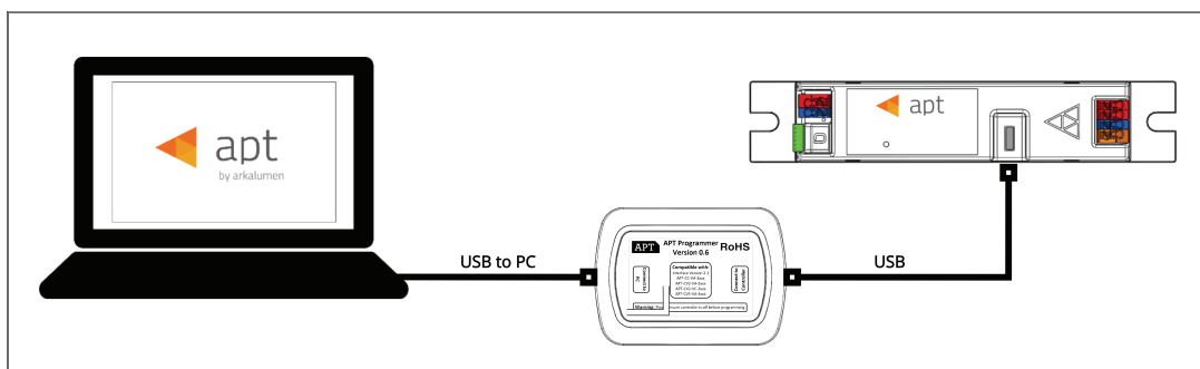
Figure 1: Wiring Diagram
