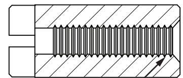
8-32 THREAD
