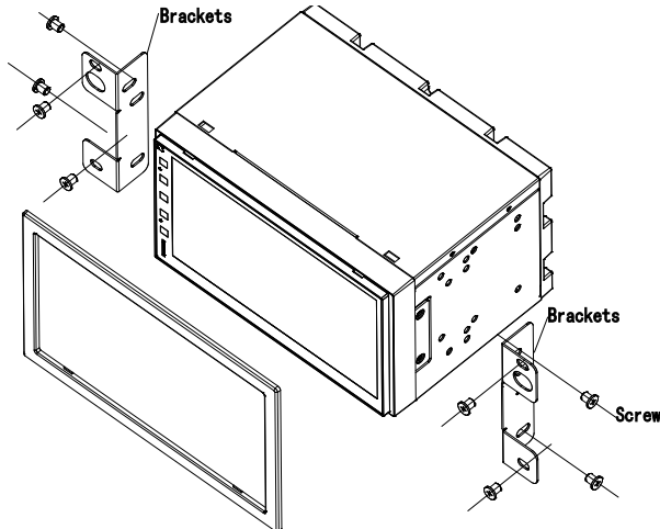
Typical front load ISO-DIN method
