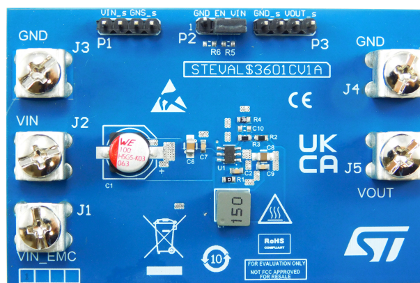
Figure 1. STEVAL-3601CV1 top view
