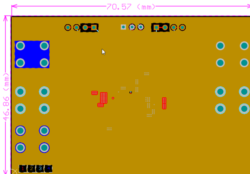
Figure 5. STEVAL-3601CV1 L1 layer
