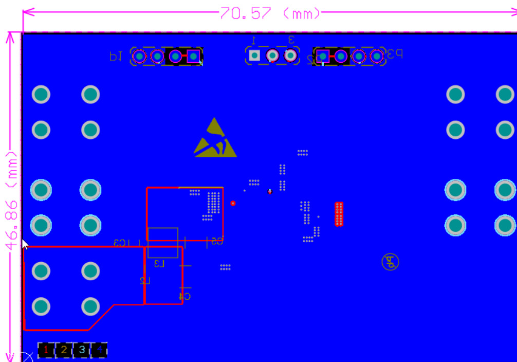
Figure 7. STEVAL-3601CV1 bottom layer
