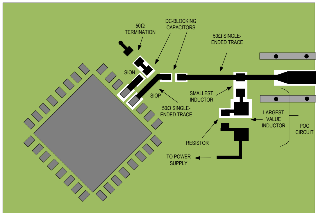
Figure 30. Coax PoC Layout Example
