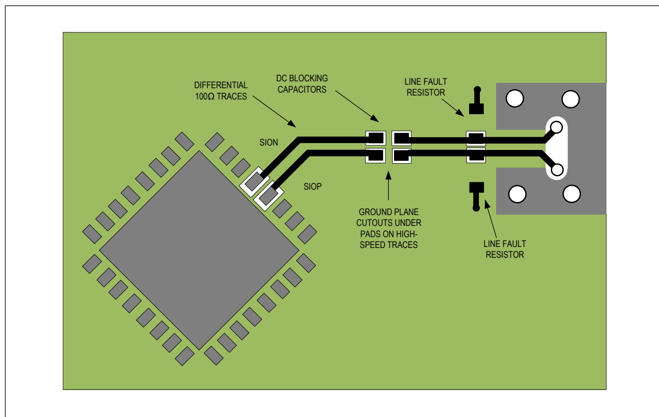
Figure 31. STP Layout Example
