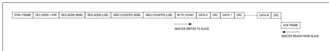
Figure 46. UART Multiple-Byte Write Transactions with CRC
