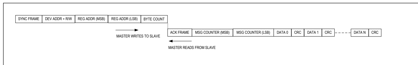
Figure 48. UART Multiple-Byte Read Transaction with CRC
