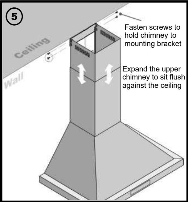
(5) To avoid scratching the chimney, extend the upper chimney slowly and carefully to the chimney-mounting bracket and tighten screws.
