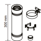
LS Flue Transition Extension Kit LSEXTKIT01
