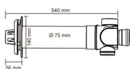
Direct Flue Kit LSFDFK01
