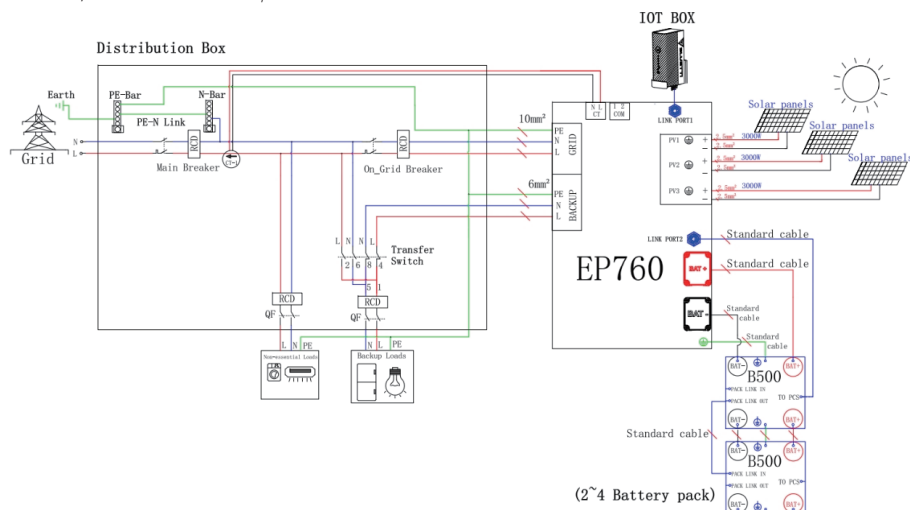
Export limitation system schematic
