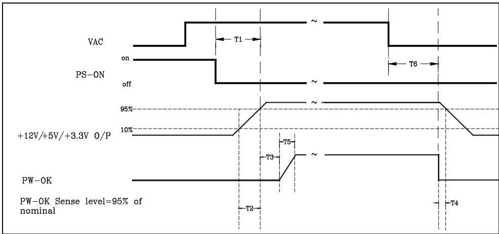
Figure 2. is a reference for signal timing for main power connector signals and rails.
