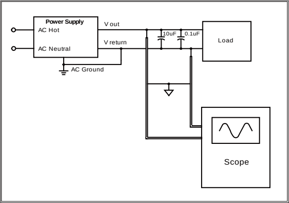
Figure 1. Ripple voltage test circuit
