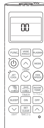
Figure 35: PQWRHQ0FDB (AKB73757604) Wireless Handheld Remote Controller for 18,000 Btu/h Cassette Indoor Units.
