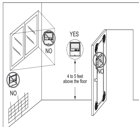
Figure 38: Proper Location for the Wired Controller.
