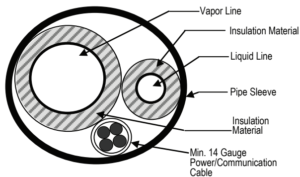
Figure 43: Typical Arrangement of Single Zone Refrigerant Pipe and Cable(s) in a Utility Conduit.
