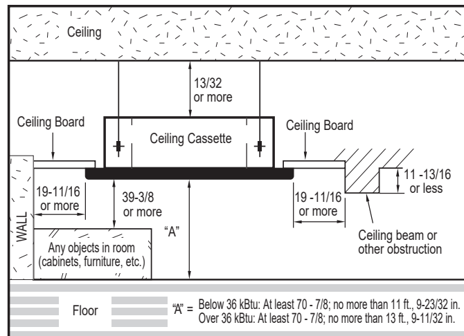
Figure 40: Indoor Unit Clearance Requirements.
