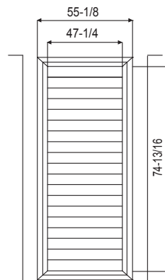
Figure 51: Example of Installing Outdoor Unit Indoors. Louver Dimensions
