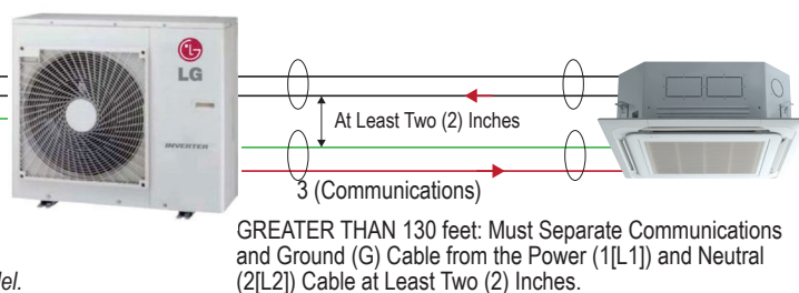
Figure 34: Schematic of a Single Zone Cassette System When the Wiring is GREATER THAN 130 Feet.
