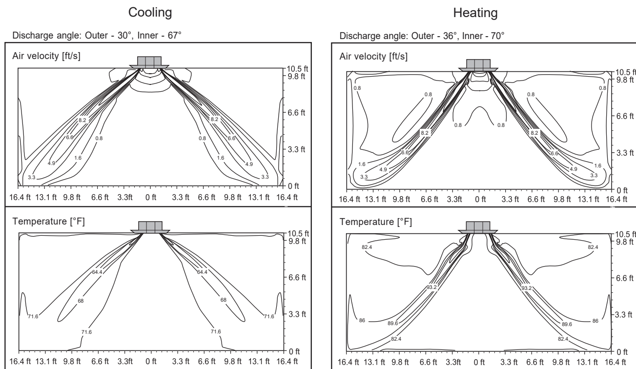
Figure 42: LCN429HV, LCN489HV Air Velocity and Temperature Distribution Charts.
