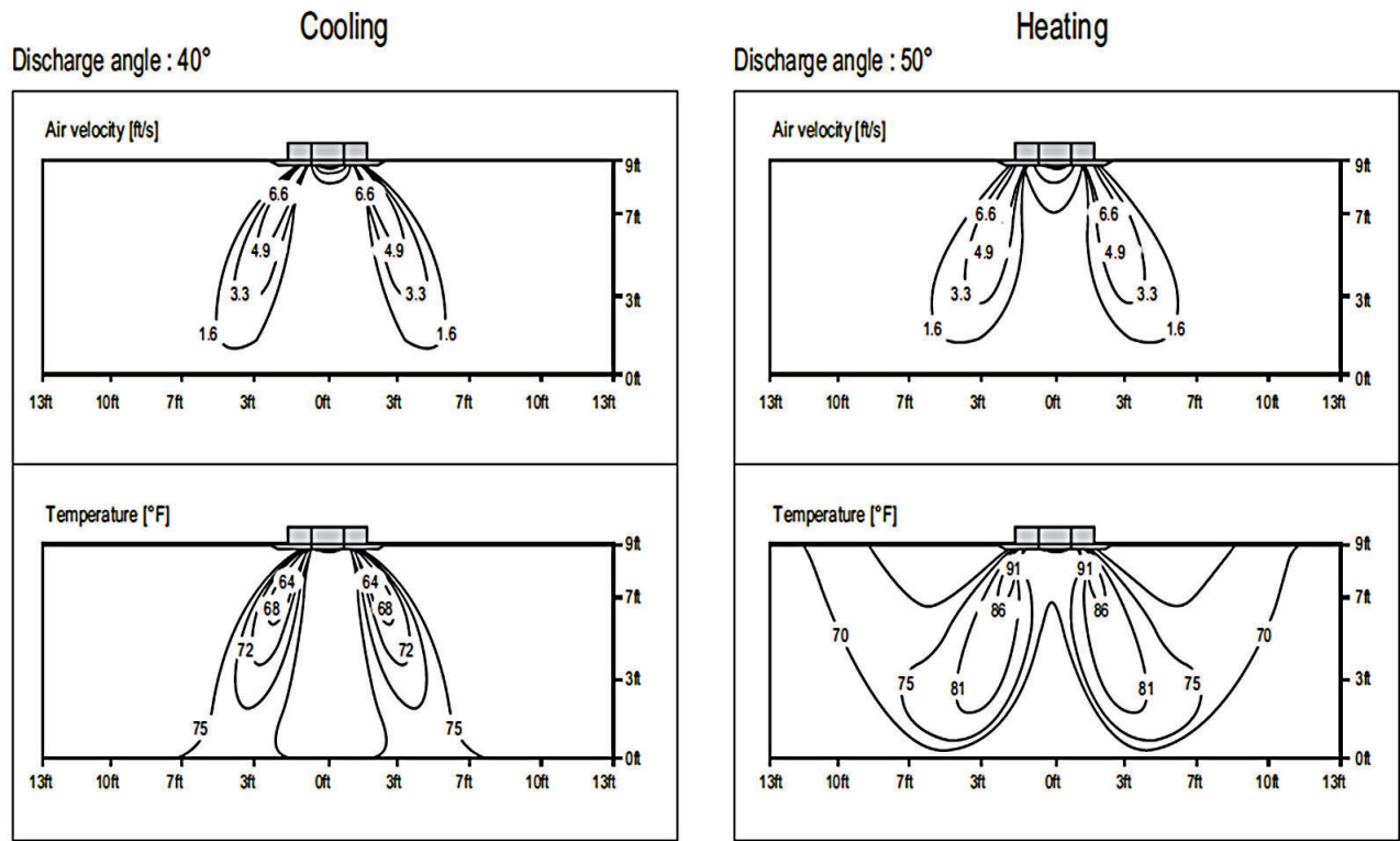
Figure 39: LCN188HV4 Air Velocity and Temperature Distribution Charts.
