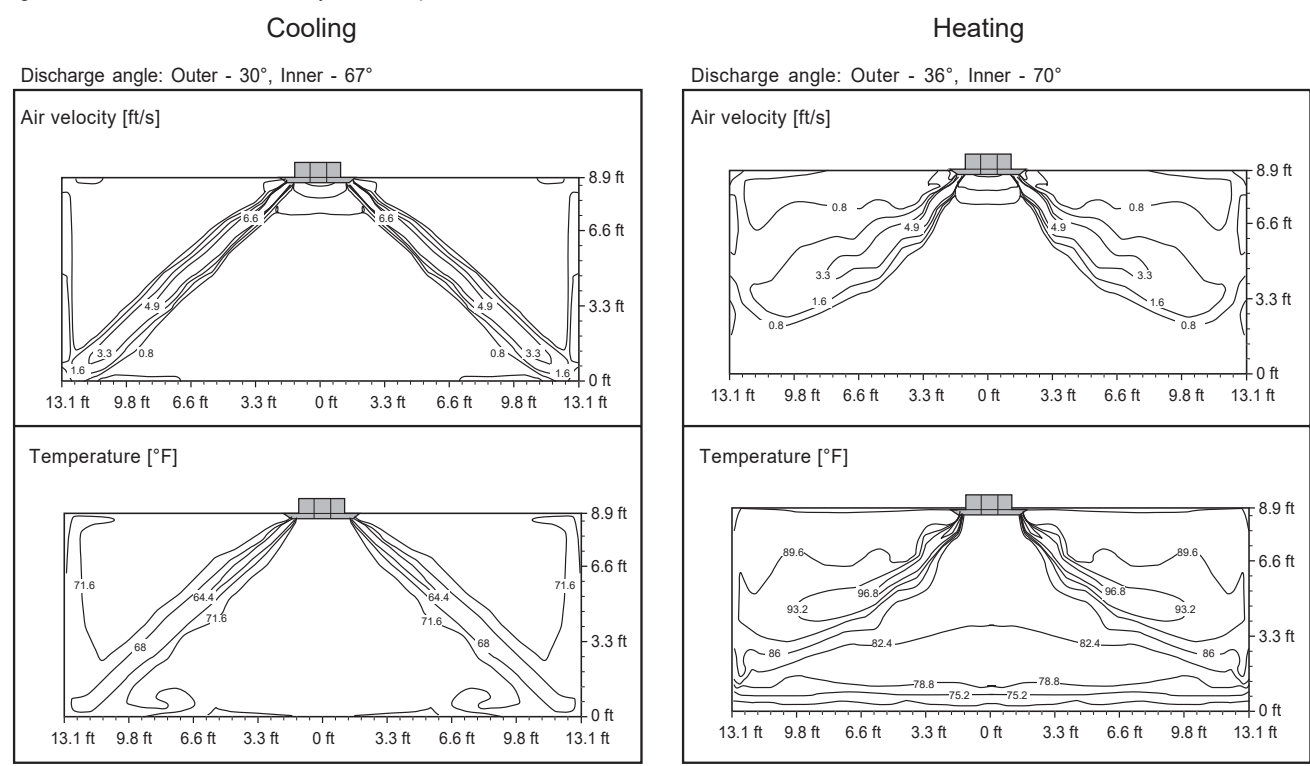
Figure 40: LCN249HV Air Velocity and Temperature Distribution Charts.
