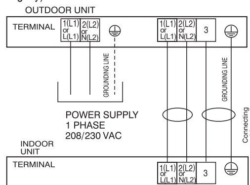
Figure 34: Schematic of a Single Zone Cassette System When the Wiring is GREATER THAN 130 Feet.
