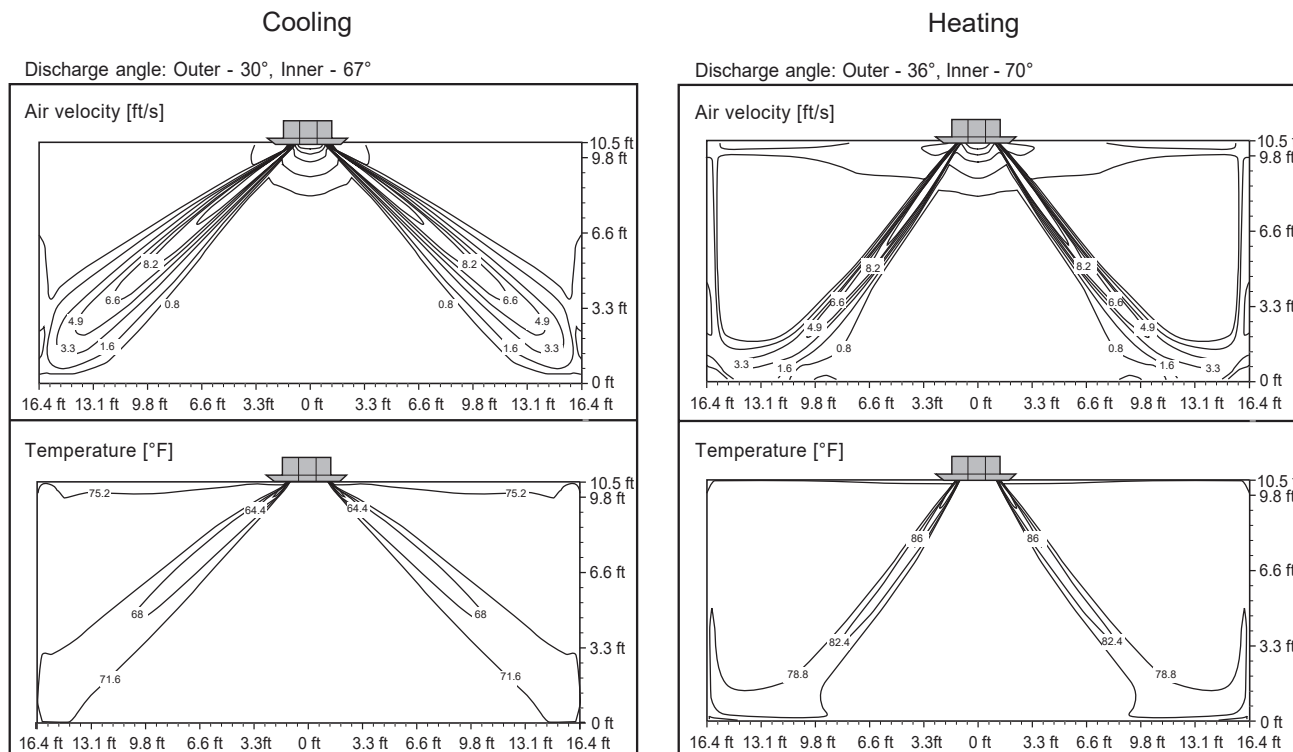
Figure 41: LCN369HV Air Velocity and Temperature Distribution Charts.
