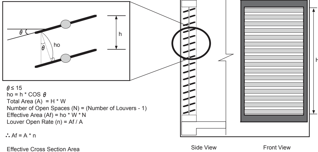
Figure 51: Example of Installing Outdoor Unit Indoors. Louver Dimensions
