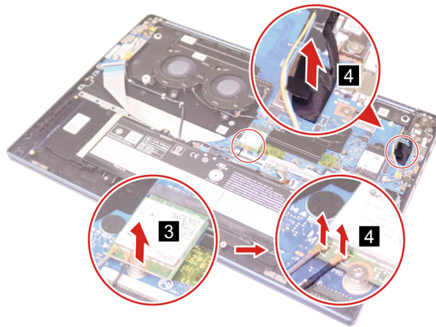
Figure 49. Disconnect antennas and EDP cable
