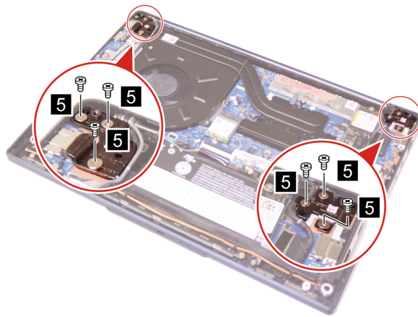
Figure 46. Remove six screws and rotate the LCD unit
