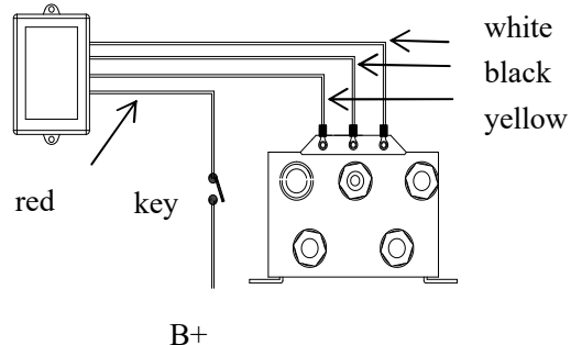
Wiring two
