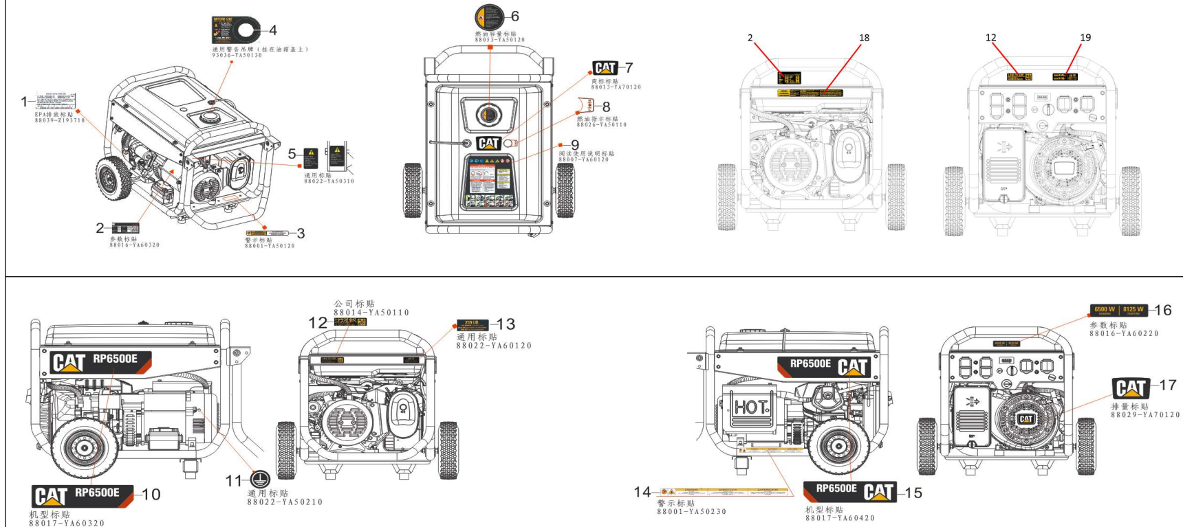
RP6500E FIG.21 DECALS/MANUAL/QSG(E00)
