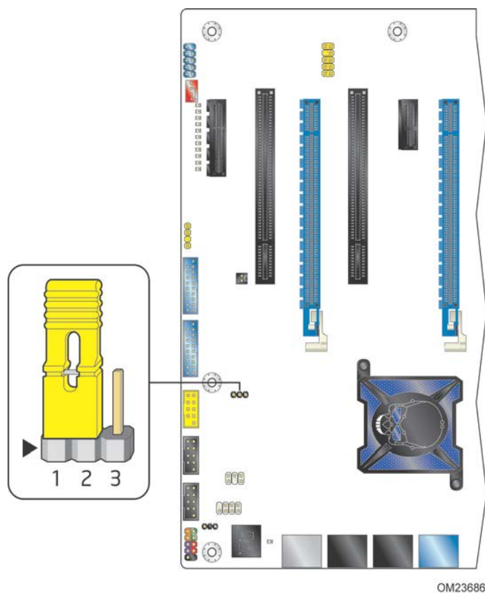
Figure 17. Location of the Jumper Block
