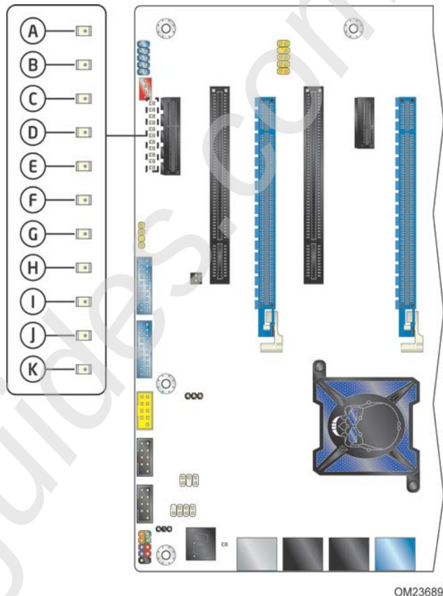
Figure 10. Location of Board Status LEDs
