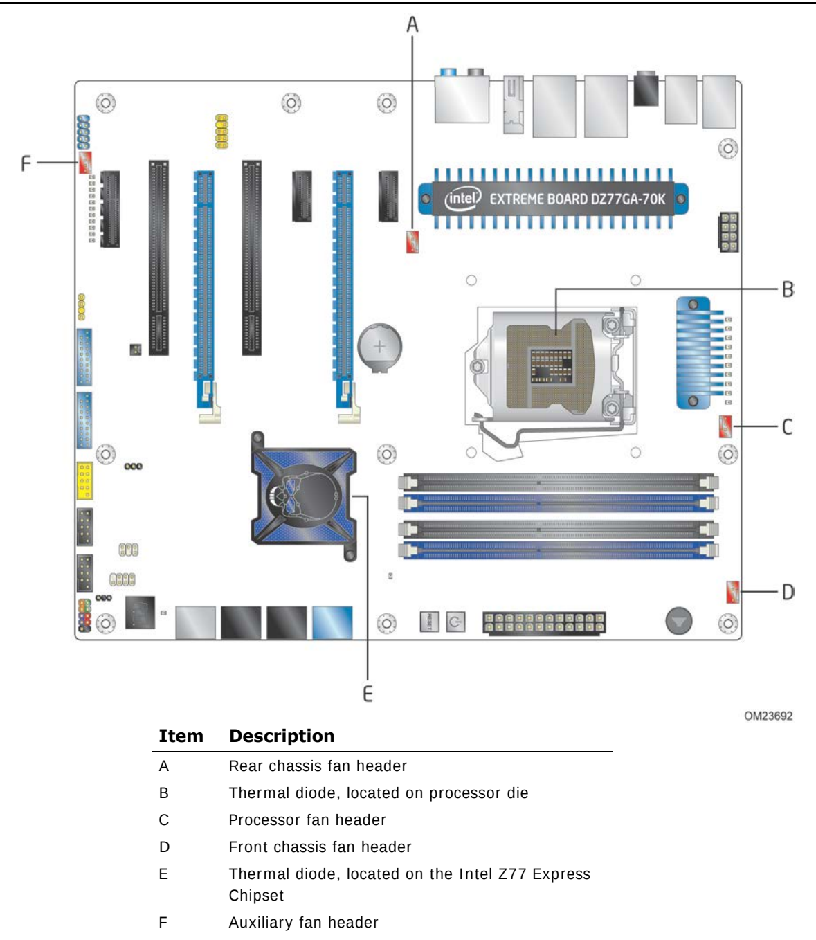
Figure 7. Thermal Sensors and Fan Headers
