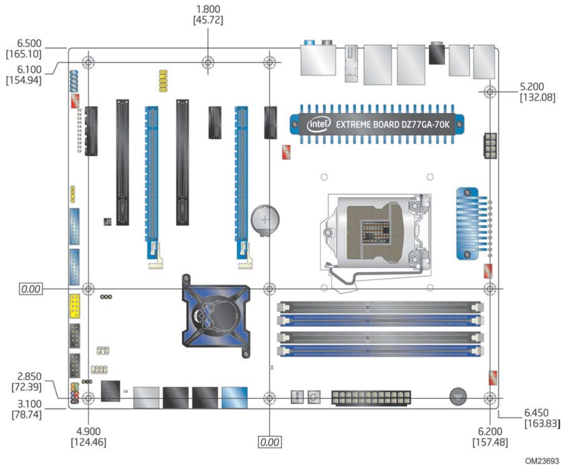
Figure 18. Board Dimensions
