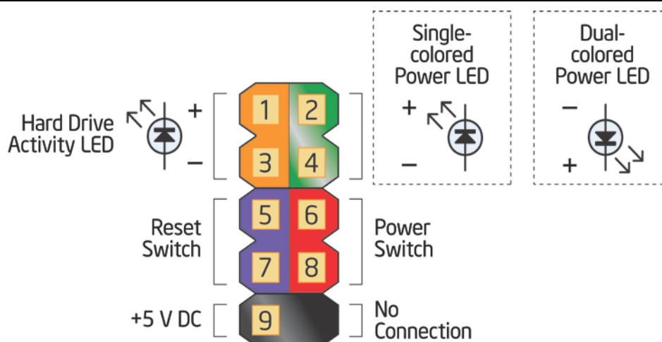
Figure 15. Connection Diagram for Front Panel Header
