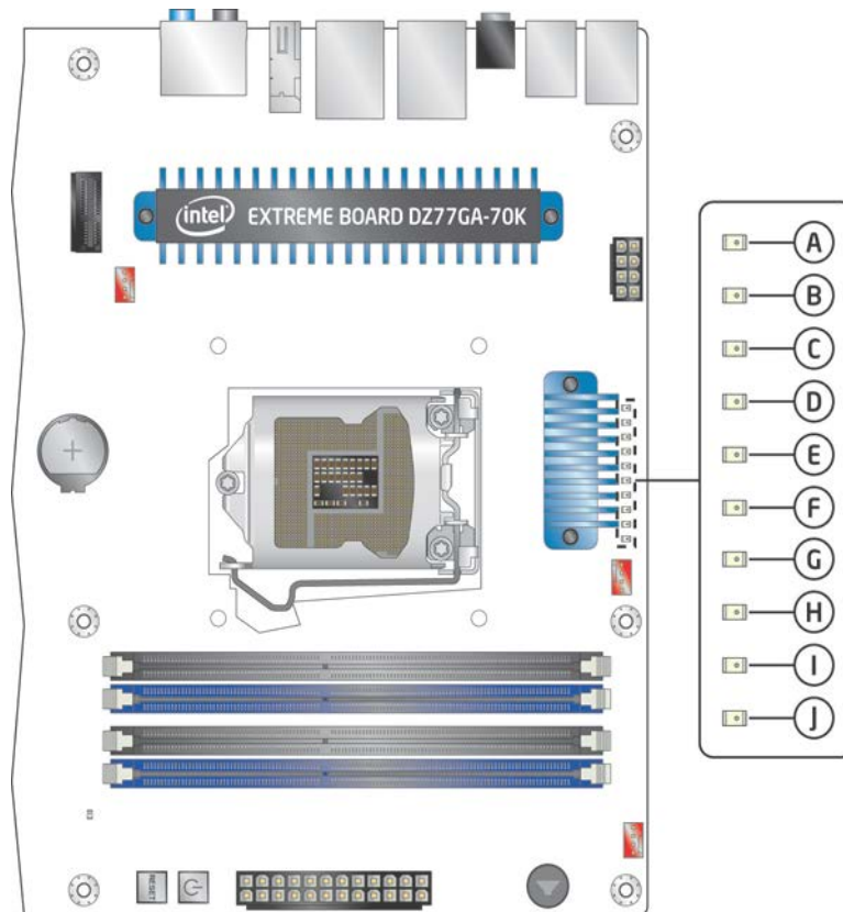
Figure 9. Location of the VR Status LEDs
