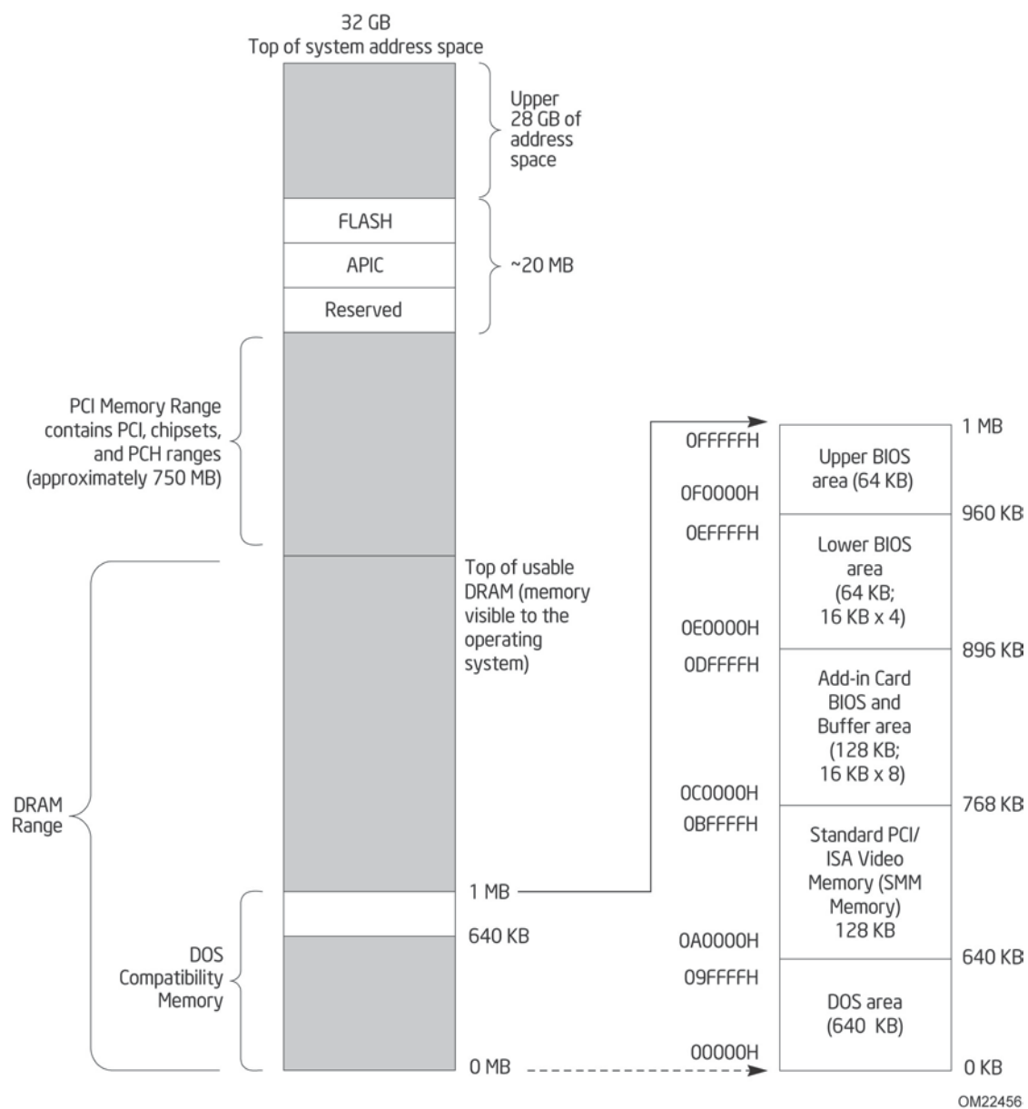
Figure 12. Detailed System Memory Address Map
