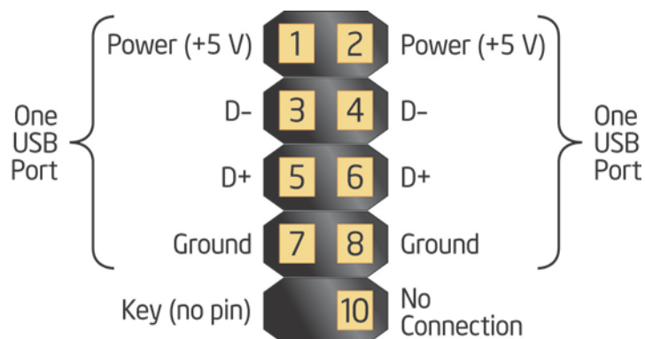
Figure 16. Connection Diagram for Front Panel USB 2.0 Headers
