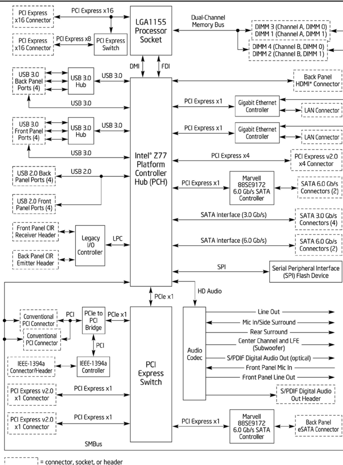
Figure 2. Block Diagram
