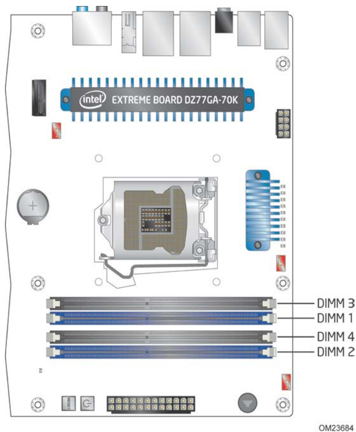
Figure 3. DIMM Configuration
