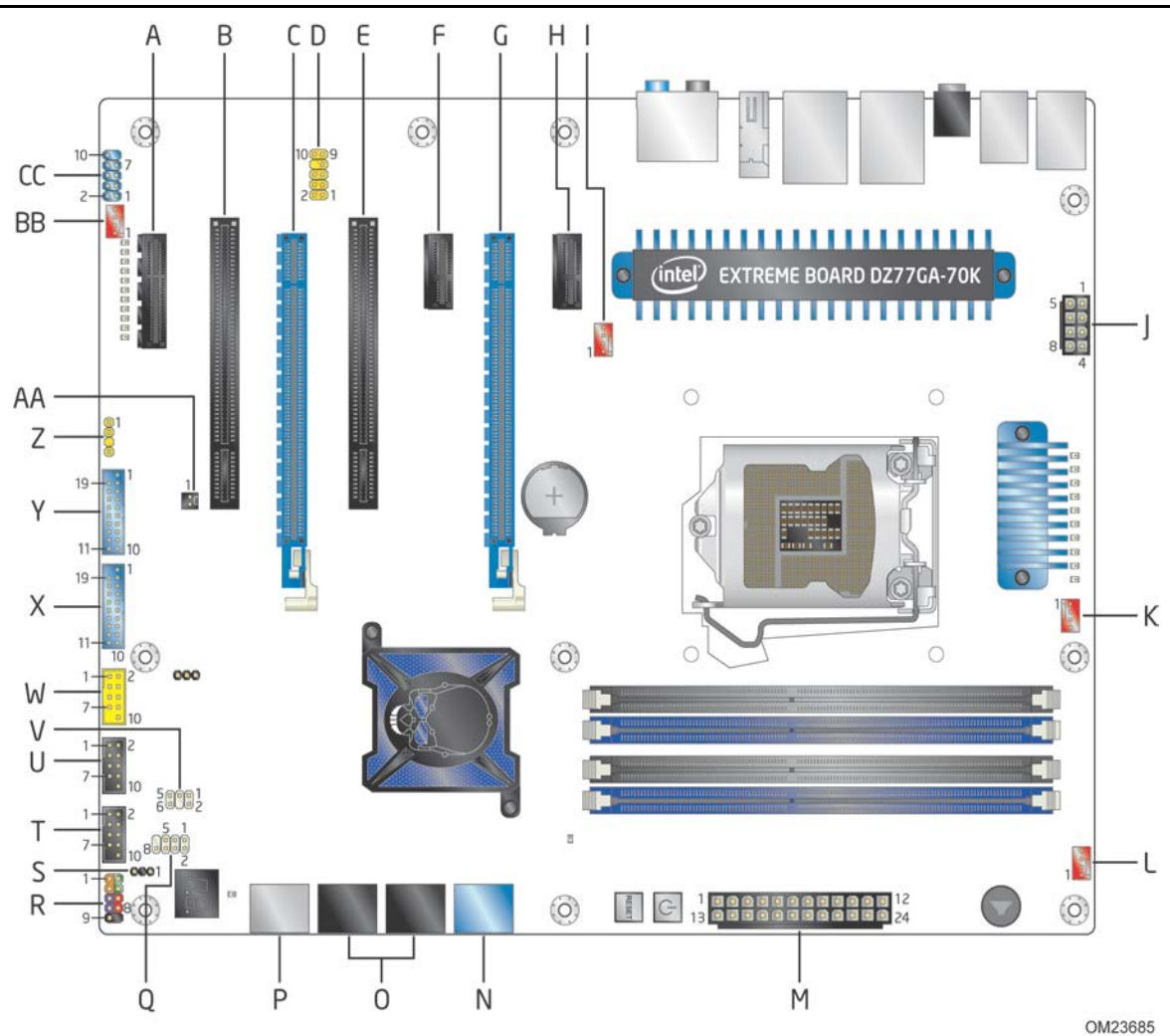
Figure 14. Component-side Connectors and Headers
