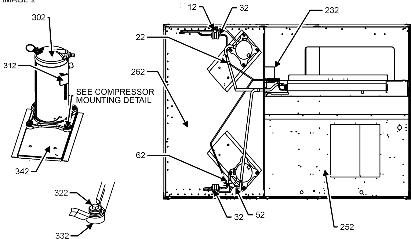
COMPRESSOR MOUNTING DETAIL
