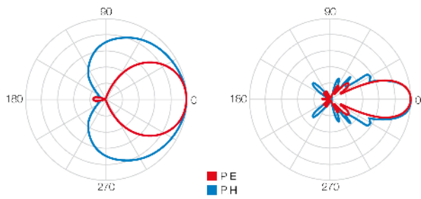
Radiation pattern
