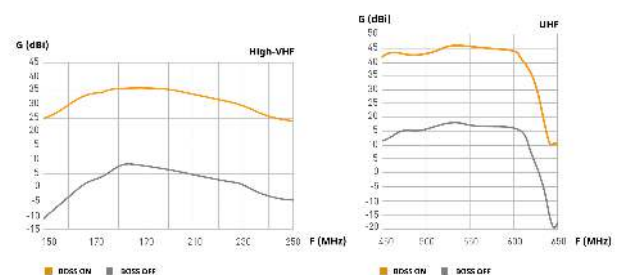
Frequency response
