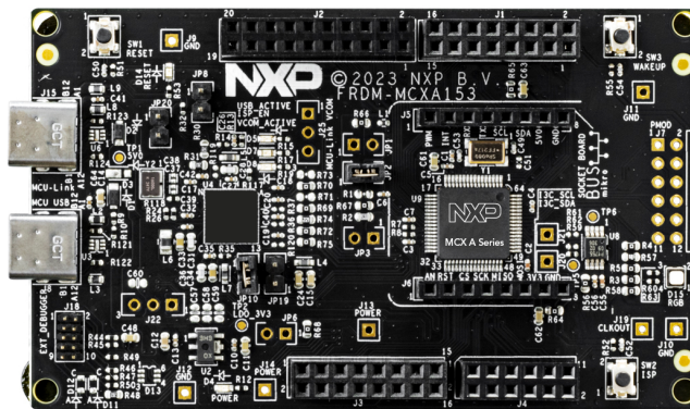
FRDM-MCXA153 FRDM Board
