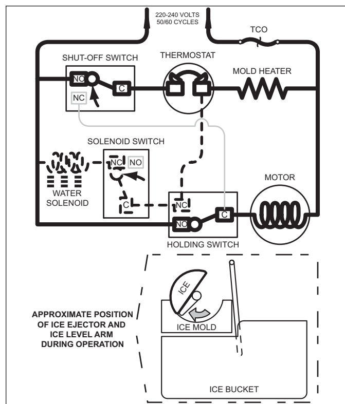
Figure 5-6. First Revolution Continued
