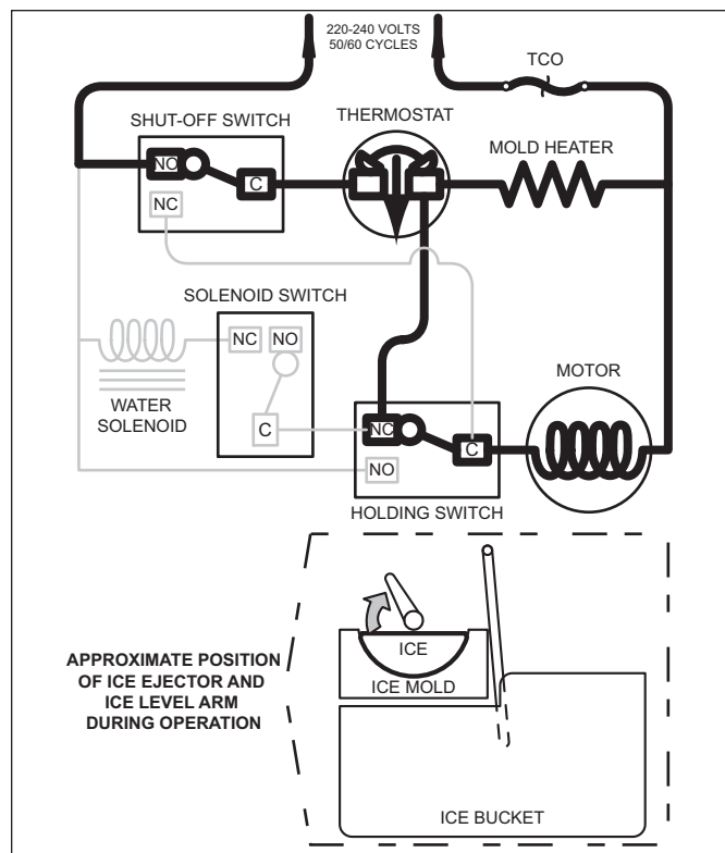
Figure 5-3. Start of First Revolution
