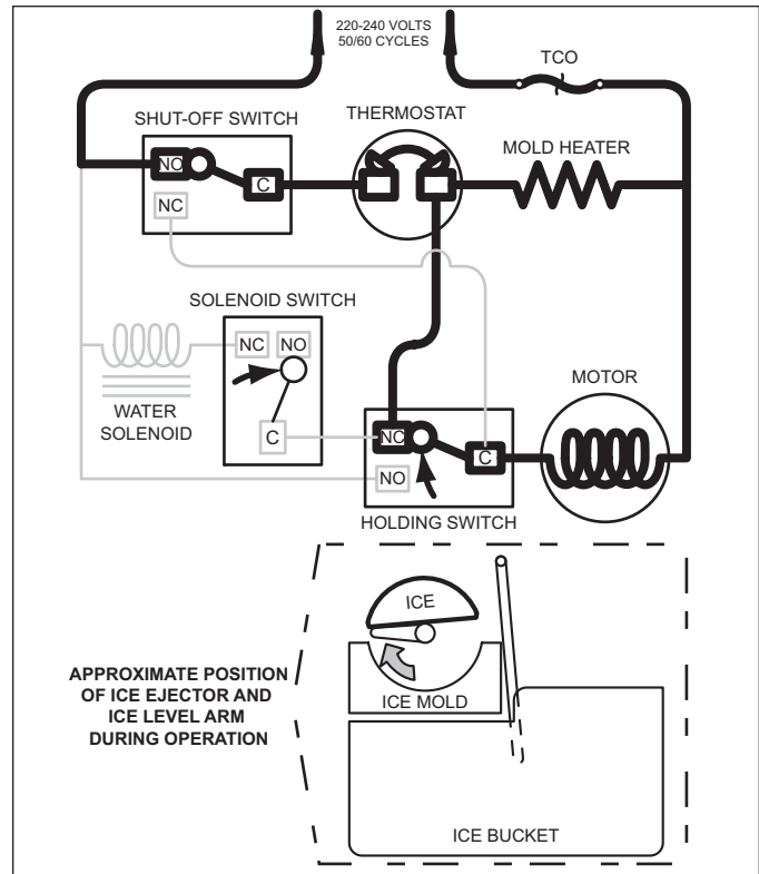
Figure 5-7. End of First Revolution
