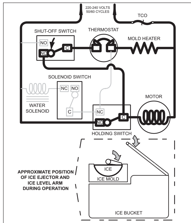
Figure 5-5. First Revolution Continued
