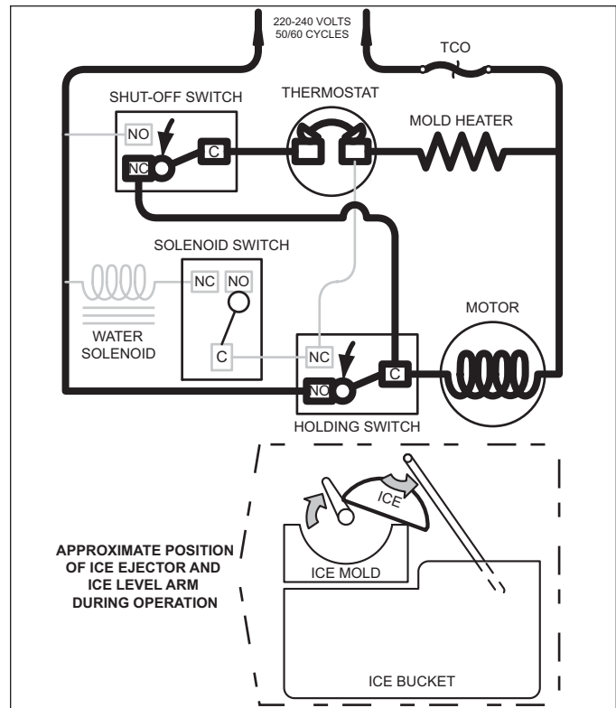
Figure 5-8. Start of Second Revolution
