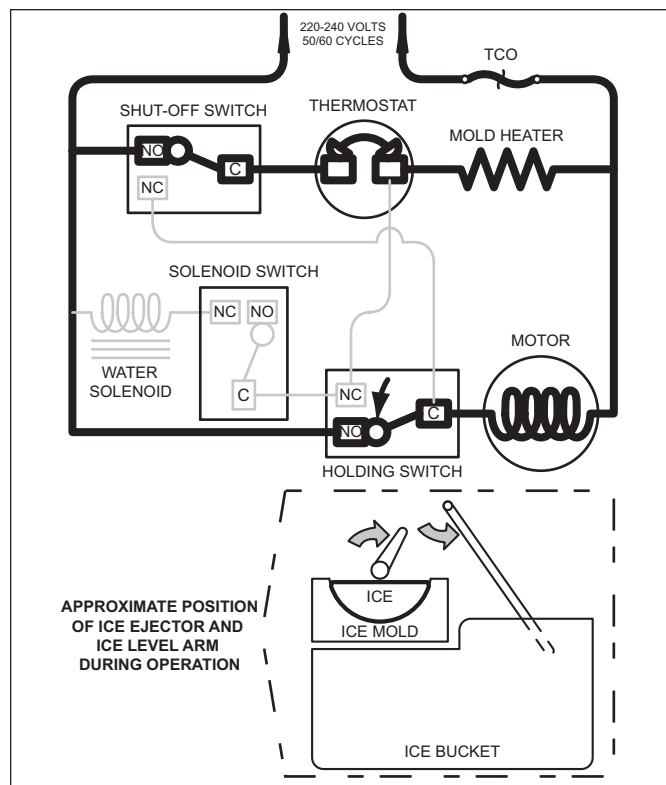
Figure 5-4. First Revolution Continued
