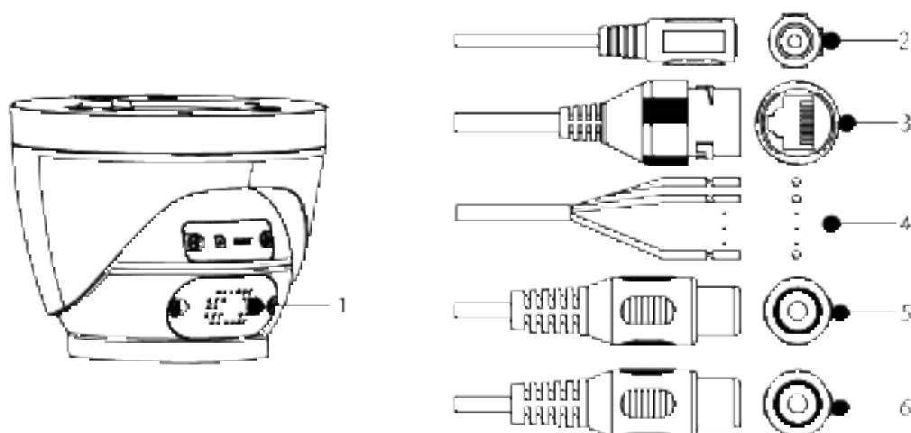
Figure 1-1 Structure components
