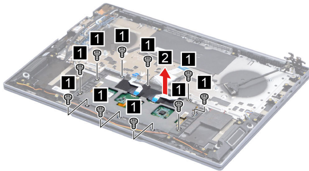
Figure 40. Remove the touchpad (type 2)
