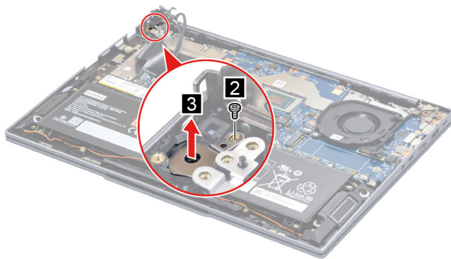
Figure 29. Remove the power button bracket
