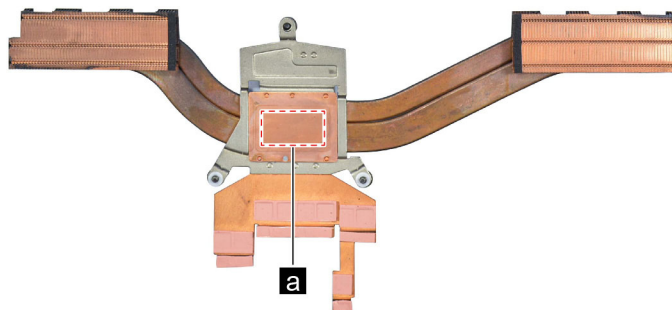
Figure 5. Areas on the heat sink where thermal interface materials should be applied
