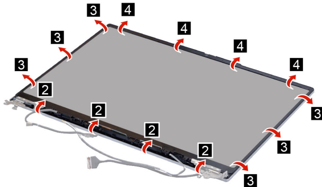
Figure 46. Remove the LCD bezel
