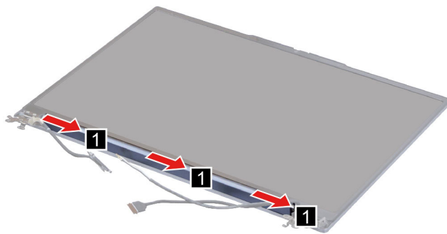
Figure 44. Remove the hinge cover
