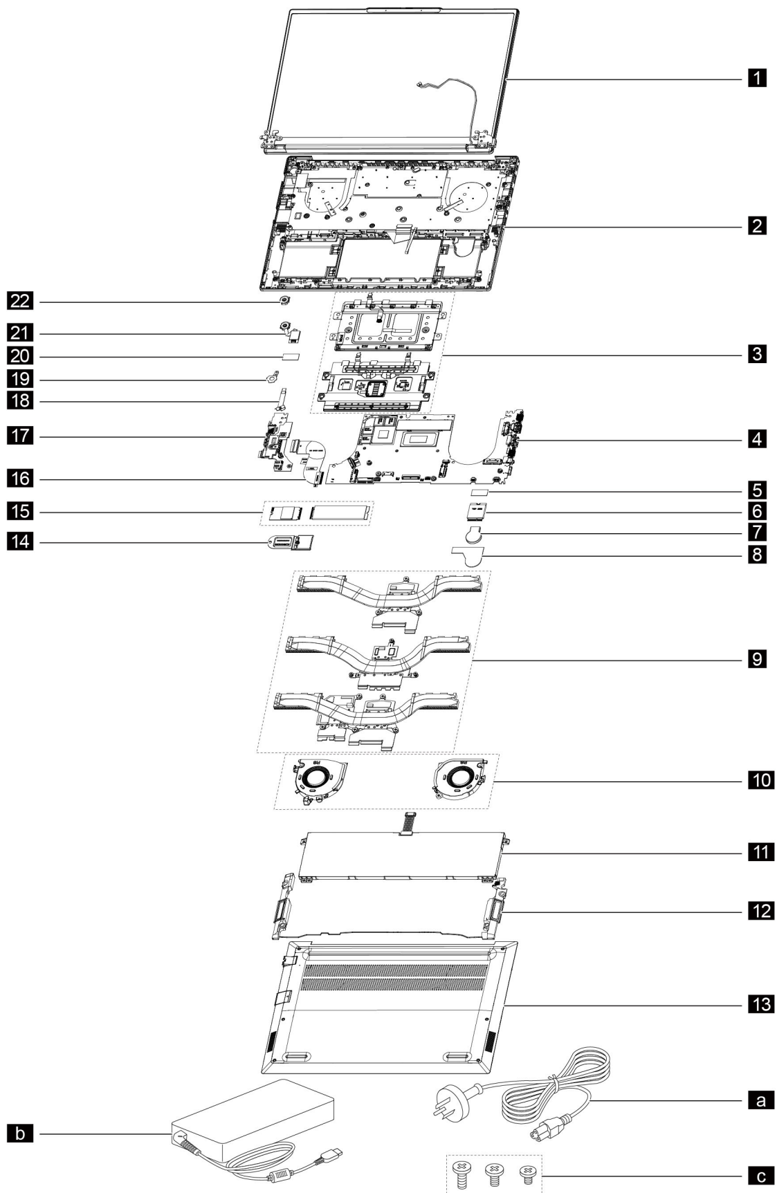
Figure 1. Exploded view
