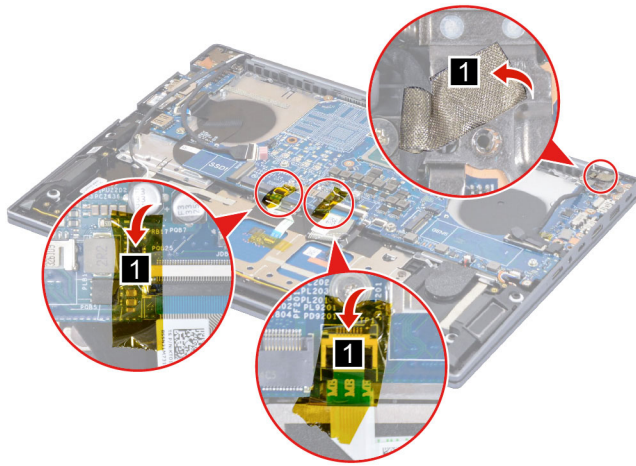
Figure 33. Peel off the three pieces of tape
