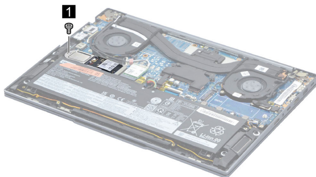
Figure 14. Remove one screw
