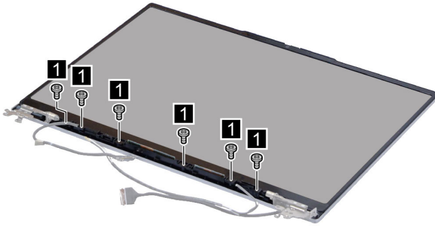
Figure 45. Remove six screws
