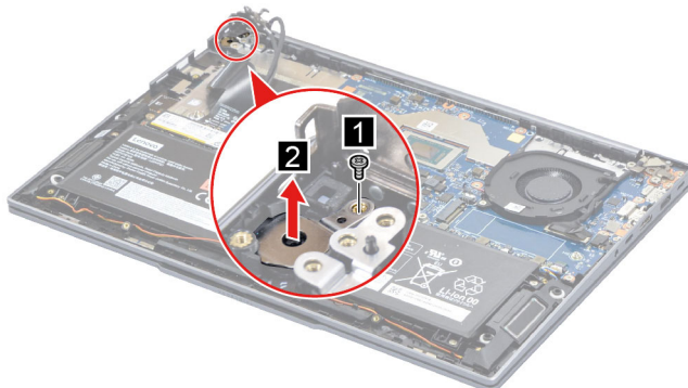
Figure 26. Remove the power button bracket
