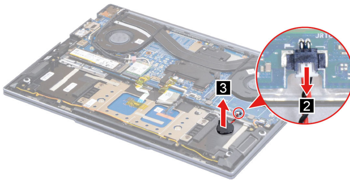
Figure 32. Remove the CMOS battery
