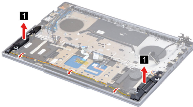
Figure 38. Remove the speakers
