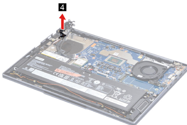
Figure 30. Remove the power button (with fingerprint board)
