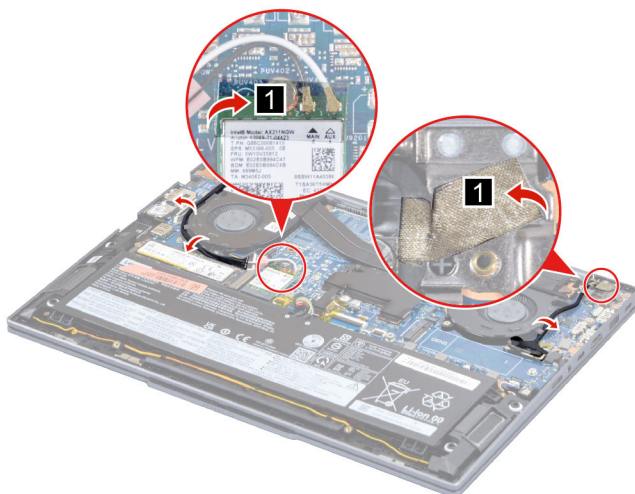
Figure 41. Peel off the tape and remove the Wi-Fi card cover
