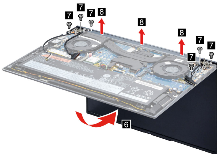
Figure 43. Remove the LCD module
