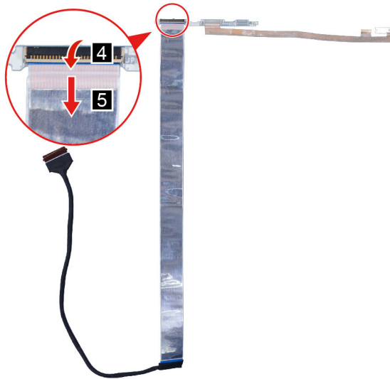
Figure 51. Remove the camera cable
