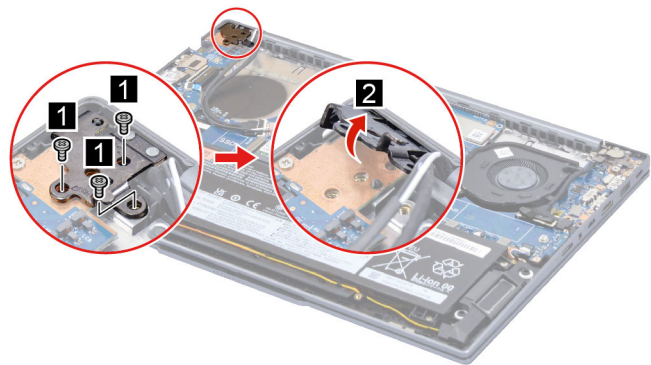
Figure 23. Remove three screws and then flip the hinge
