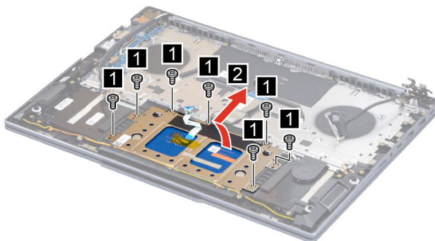
Figure 39. Remove the touchpad (type 1)
