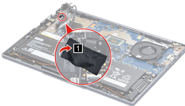
Figure 28. Peel off the acetate tape
