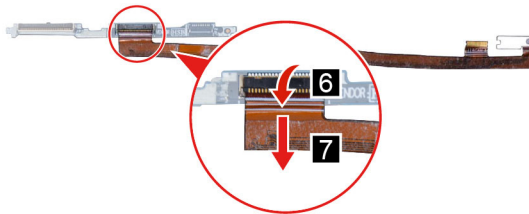
Figure 52. Remove the sensor board cable
