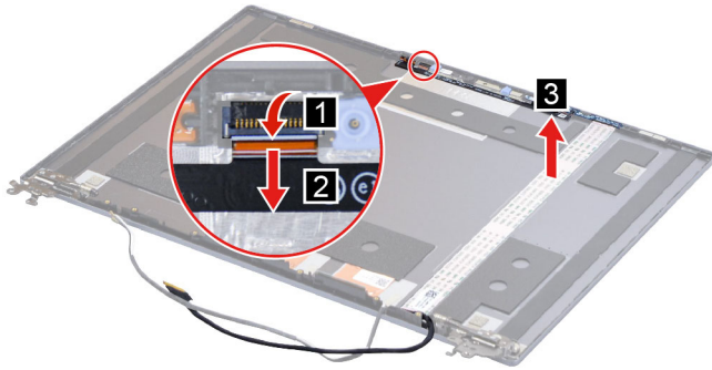
Figure 50. Remove the sensor board module
