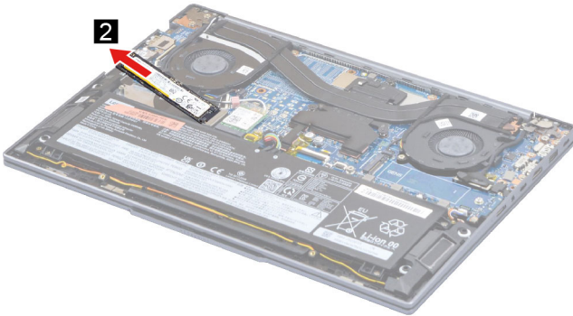
Figure 13. Remove the SSD
