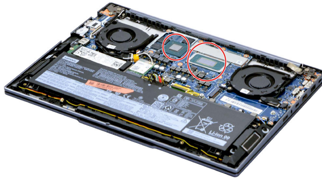
Figure 8. Areas on the system board where thermal interface materials are applied
