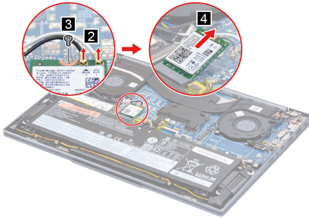
Figure 18. Remove the Wi-Fi card
