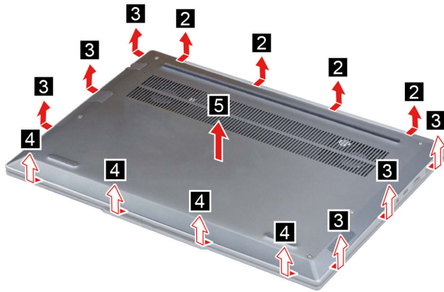
Figure 10. Remove the lower case
