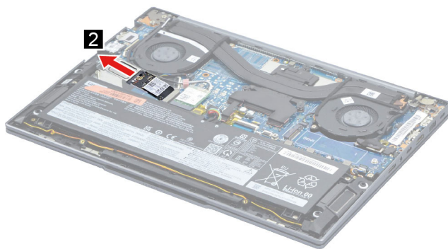
Figure 15. Remove the SSD
