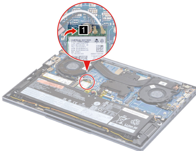
Figure 17. Remove the Wi-Fi card cover
