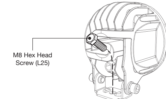
M8 Hex Head Screw (L25) M8 Washer M8 Spring Washer M8 Nut
