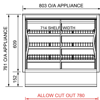
FRONT ELEVATION
