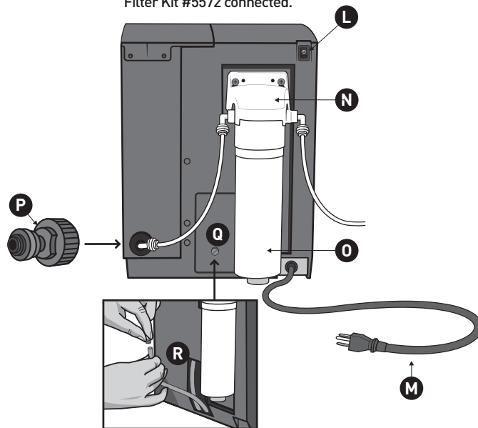
Back view with optional Filter Kit #5572 connected.
