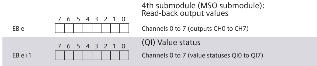
Figure 5-3 Address space for configuration as 1 x 8-channel DQ 8x24VDC/0.5A HF V1.0, MSO
