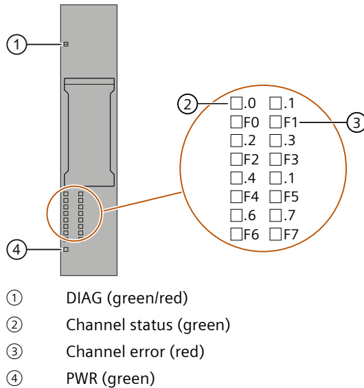
Figure 6-1 LED displays
