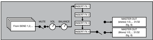
Fig. 5: SUBMIXES (Stereo)
