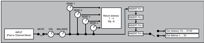
Fig. 5: SUBMIXES (Stereo)
