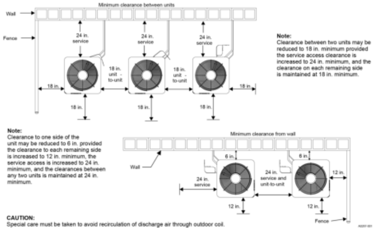
Figure 5: Alternative installation clearances
