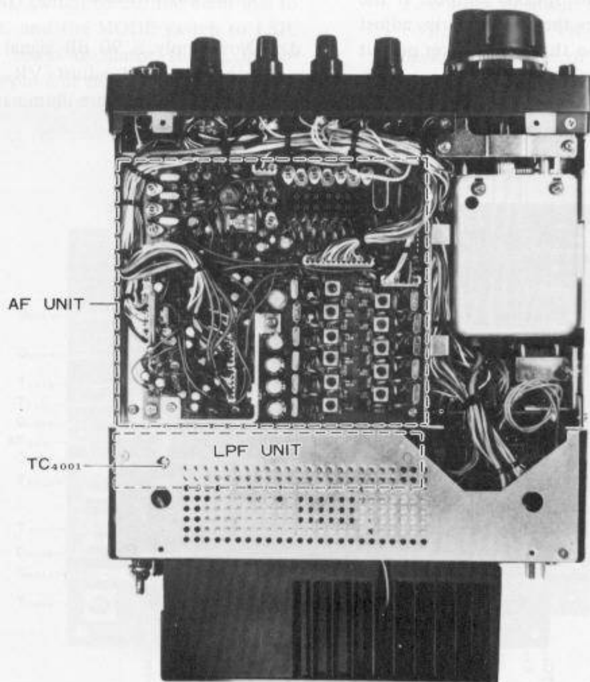
BOTTOM VIEW
