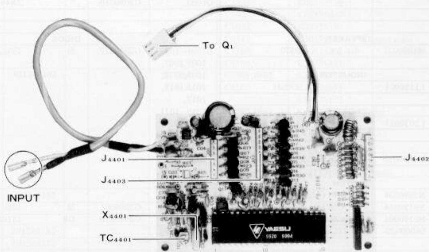
COUNTER UNIT
