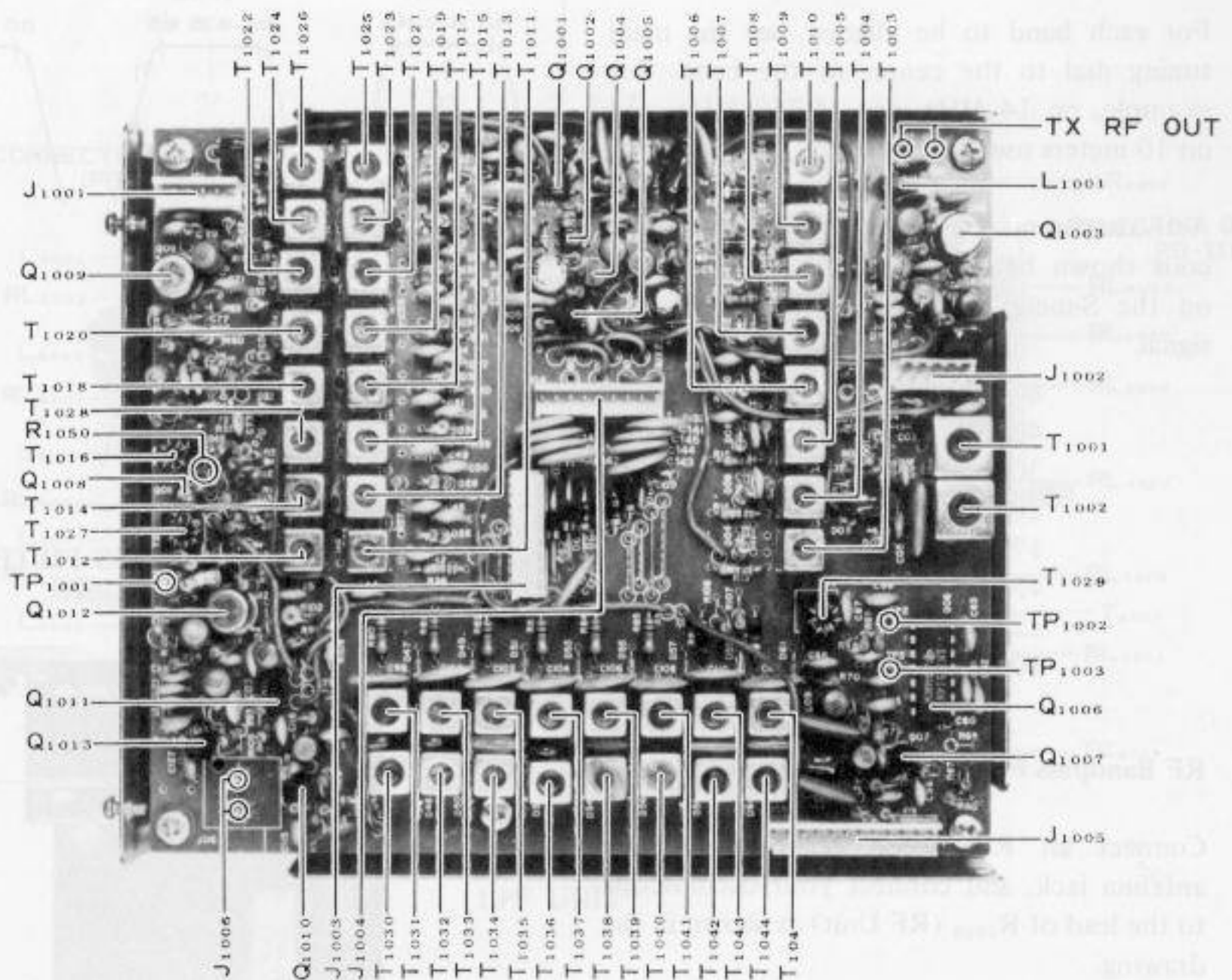
RF UNIT
