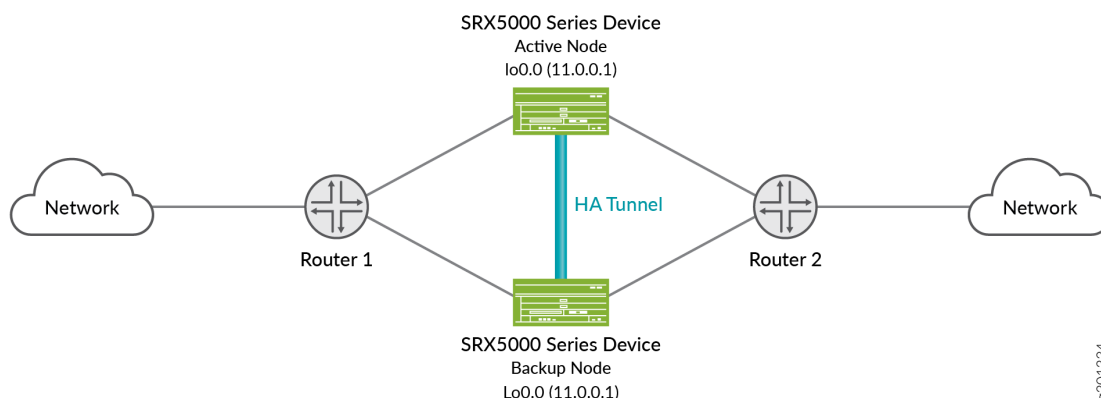
Figure 39: Active/backup Nodes With Floating IP Address
