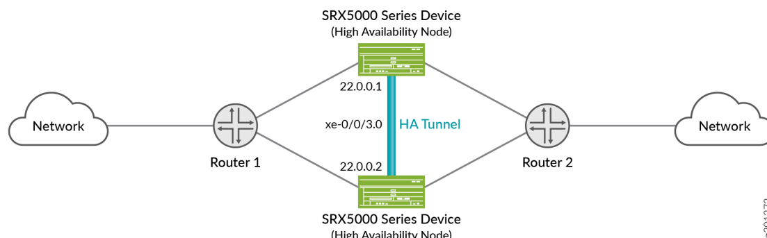
Figure 40: High Availability Tunnel Link Encryption
