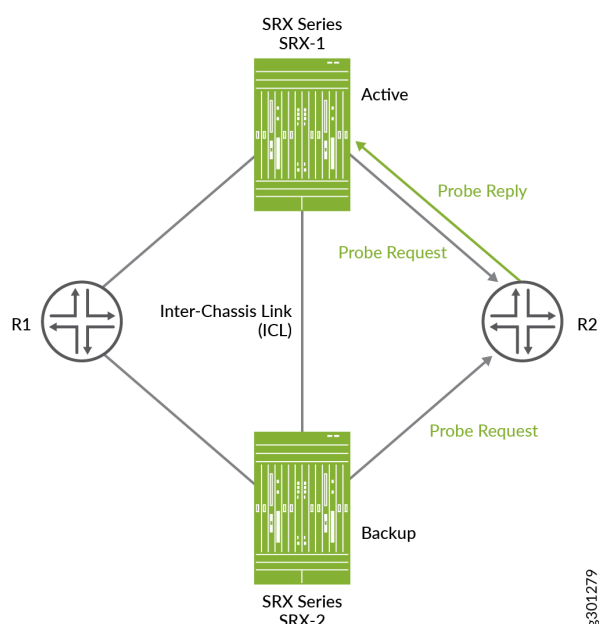
Figure 38: Deployment of Multinode High Availability in Active/Backup Mode
