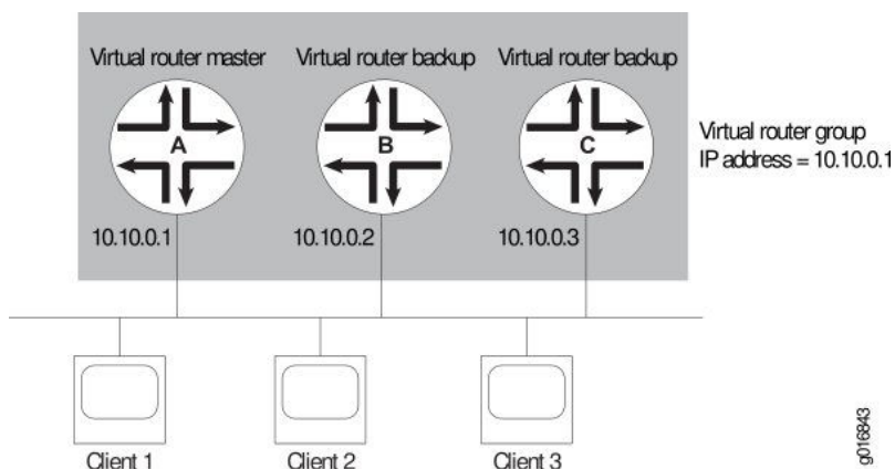
Figure 25: Basic VRRP
