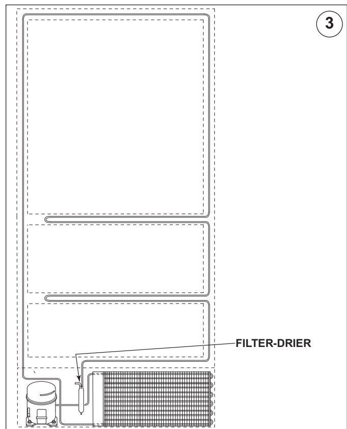
Figure 4-3. Filter-Drier
