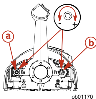
a - Detent tension adjustment screw b - Control handle tension adjustment screw
