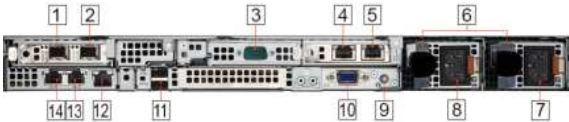
Figure 3-6: DMF Analytics Node (DCA-DM-AN450) Rear Panel
