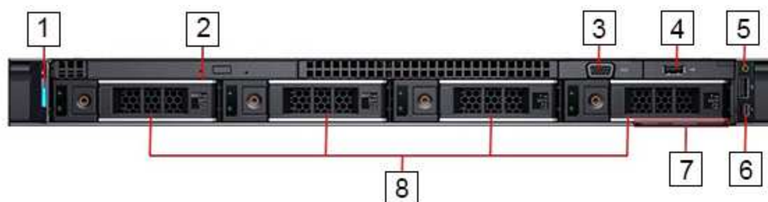
Figure 3-2: Arista Analytics Node (DCA-DM-AA/DCA-DM-AA2/DCA-DM-AA3) Front Panel
