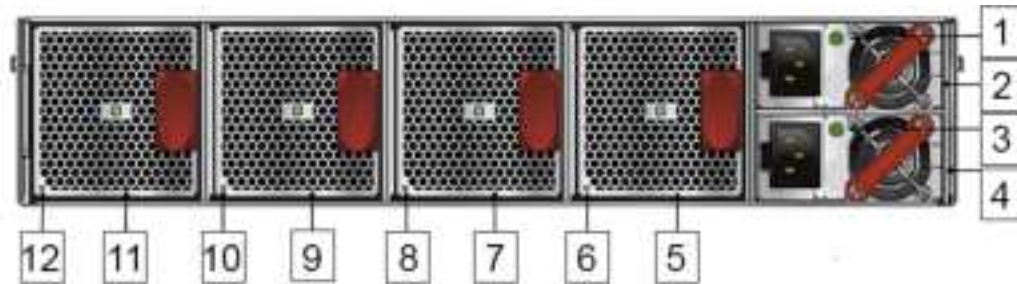
Figure 5-12: Port and Environmental LEDs (Rear Panel)
