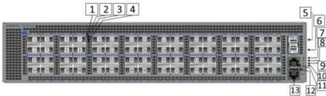
Figure 5-9: Port and Environmental LEDs (Front Panel)
