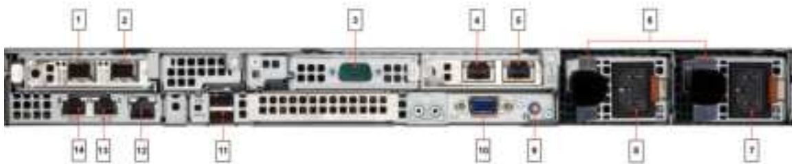
Figure 1-9: DMF Controller Node (DCA-DM-C450) Rear Panel
