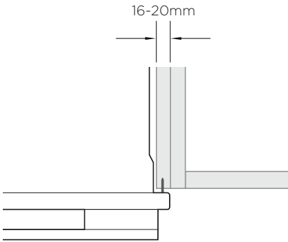
PROUD INSTALL
