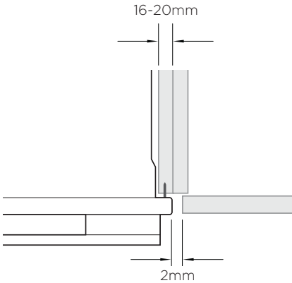
FLUSH INSTALL
