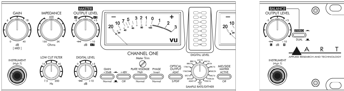
Figure 2 – Front controls
