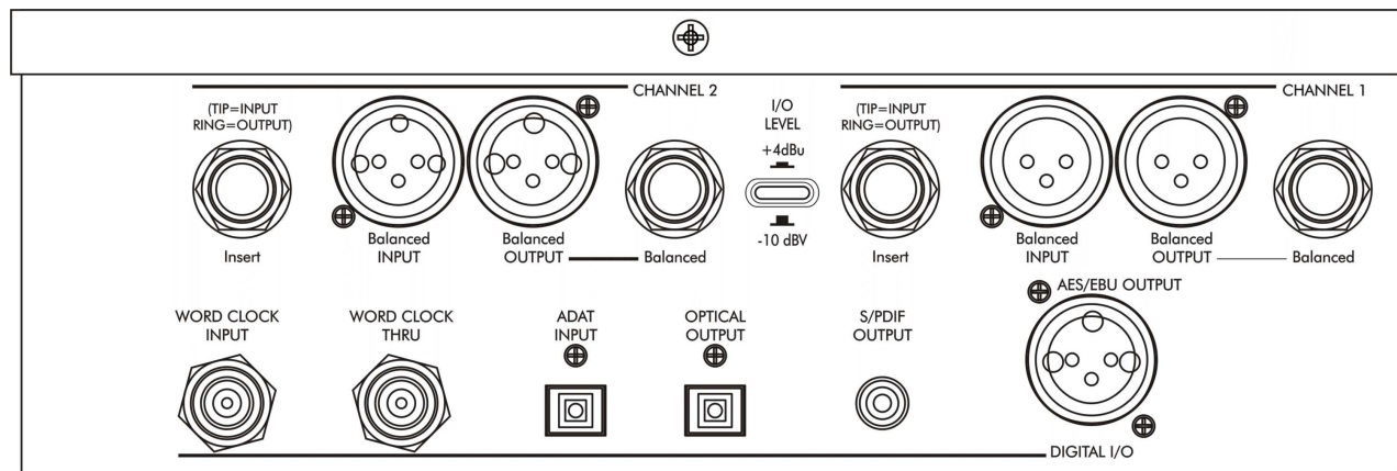
Figure 3 – Rear connections
