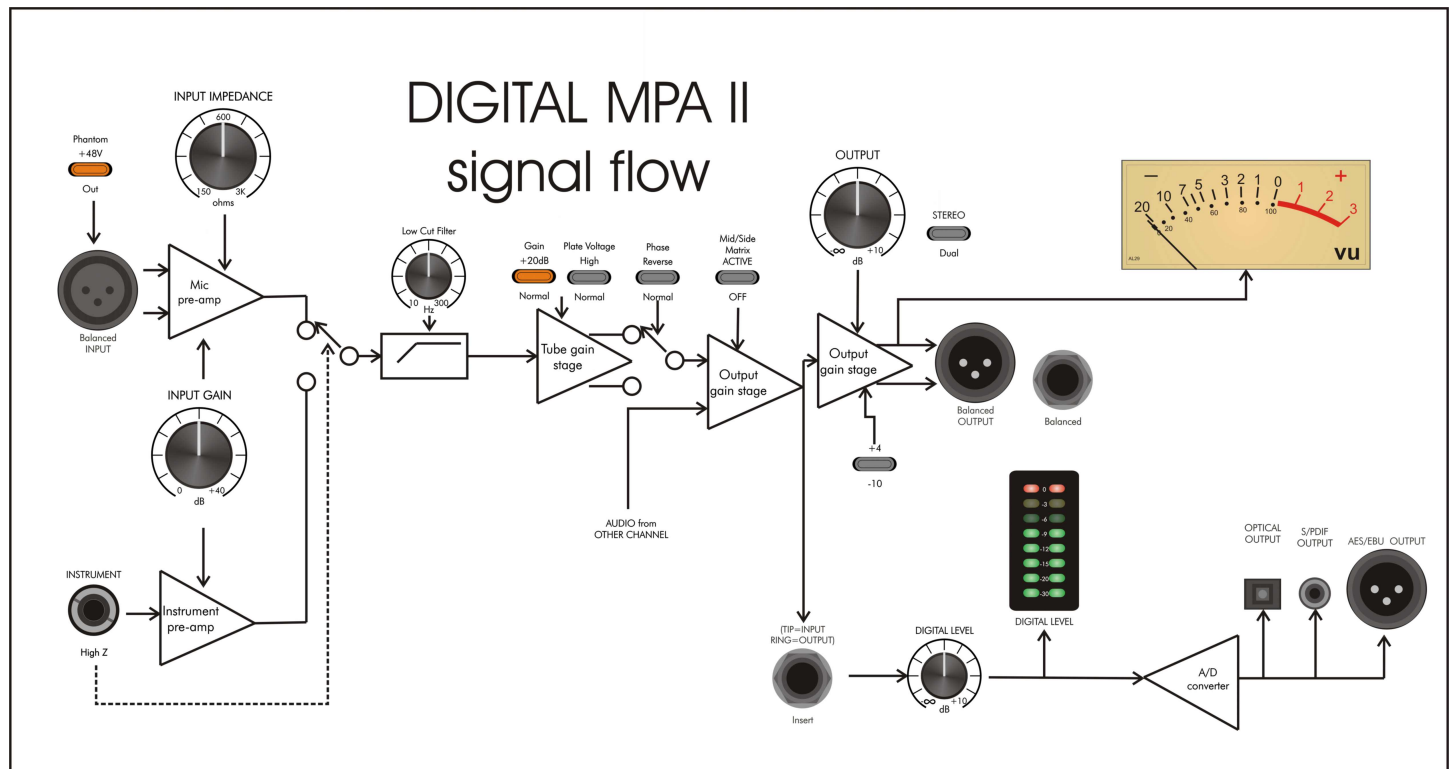
Figure 1 – Block Diagram
