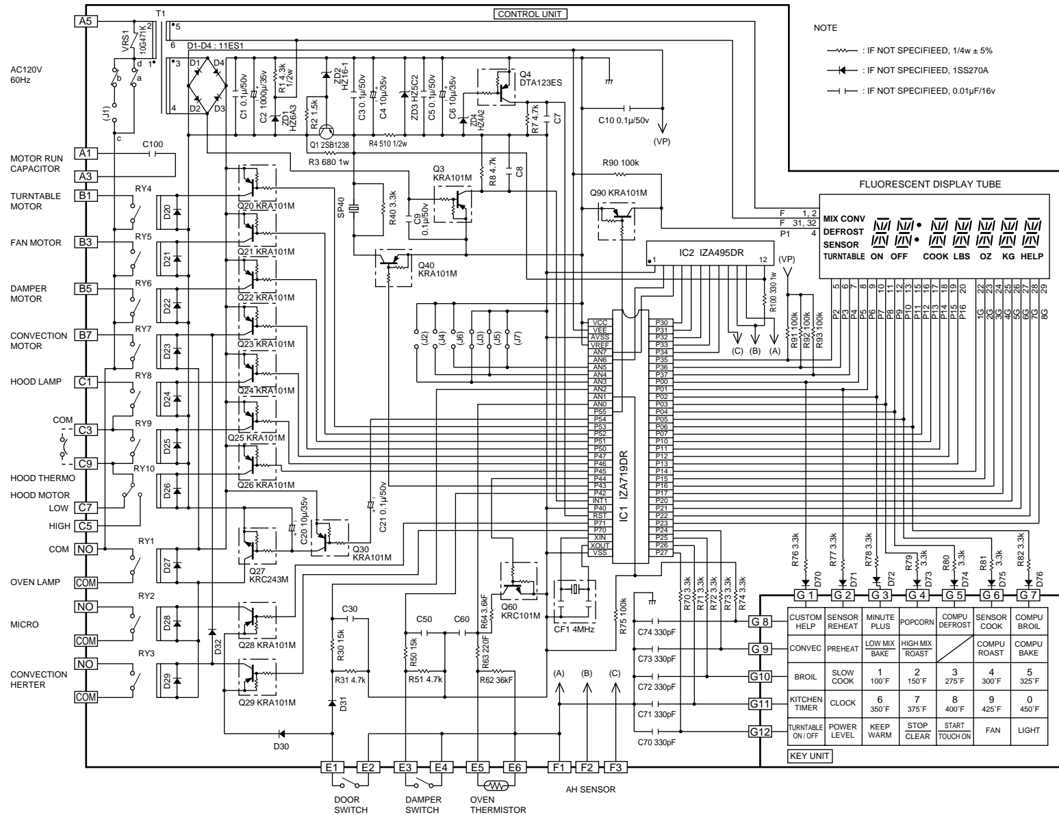
Figure S-2. Touch Control Panel Circuit
