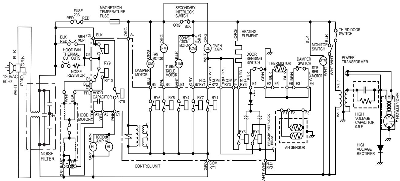
Figure O-3. Oven Schematic - Convection Cooking Condition (CONVEC, PREHEAT, BROIL, SLOW COOK)
