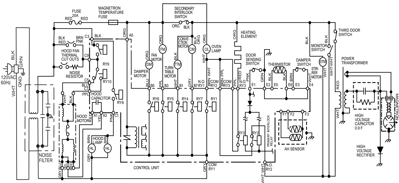
Figure O-4. Oven Schematic - Automatic Mix cooking Condition
