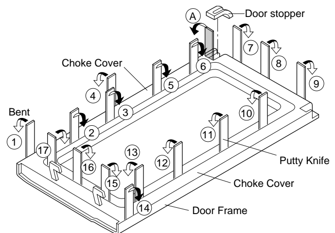
Figure C-3. Door Disassembly
