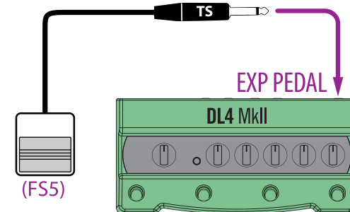
Connecting a single footswitch (TS cable connection)
