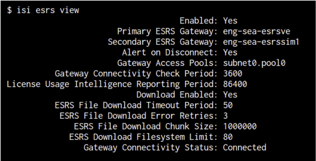
Figure 2. The isi esrs view command output
