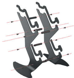
Figur 1. Monteringsillustration.
