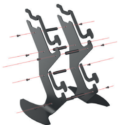
Fig 1. Assembly illustration.
