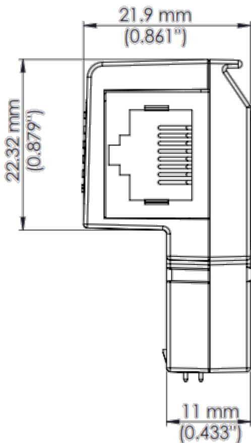
Side View
