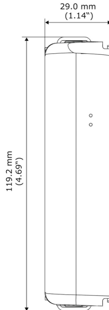
Front View
