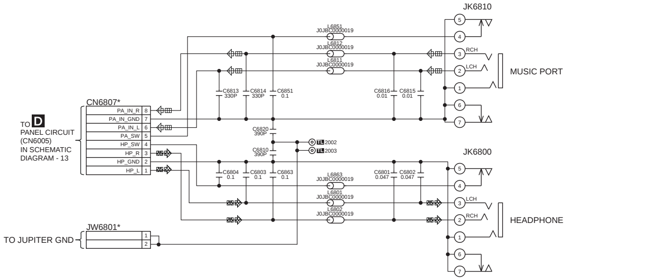
SA-AKX30PH/PN CD OPEB BUTTON / REMOTE SENSOR / TUNER / MUSIC PORT/HEADPHONE CIRCUIT
