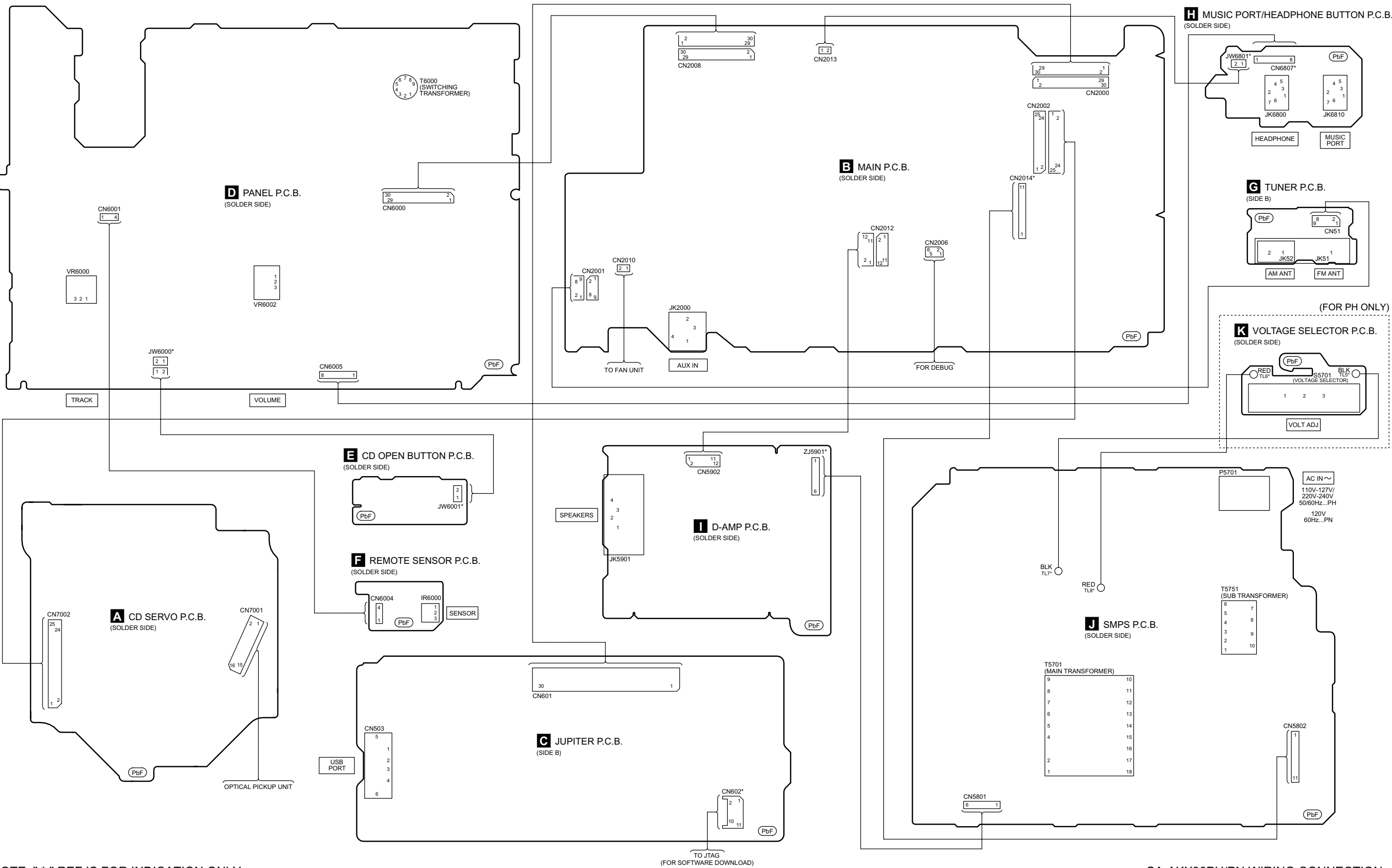
SA-AKX30PH/PN WIRING CONNECTION
