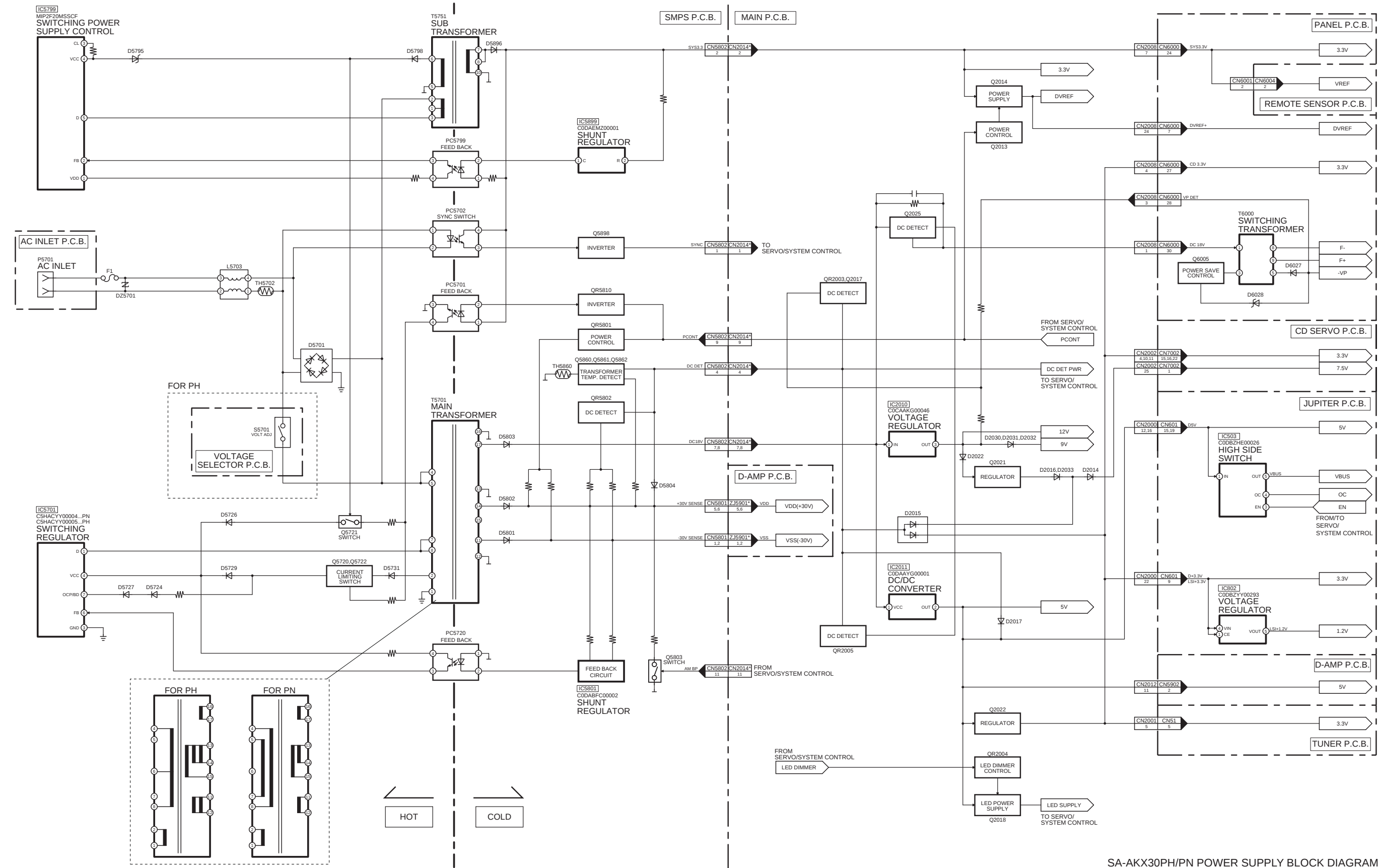
SA-AKX30PH/PN POWER SUPPLY BLOCK DIAGRAM
