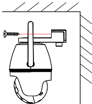
Figure 2-4 Wall-mounted installation
