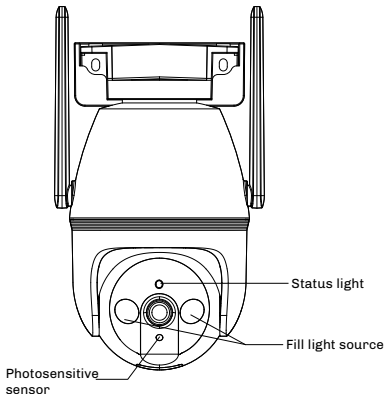
Figure2-3 structure
