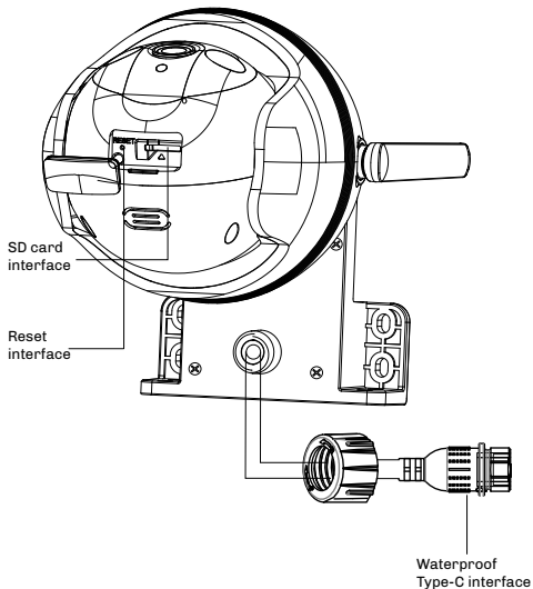
Figure 2-2 Camera ports
