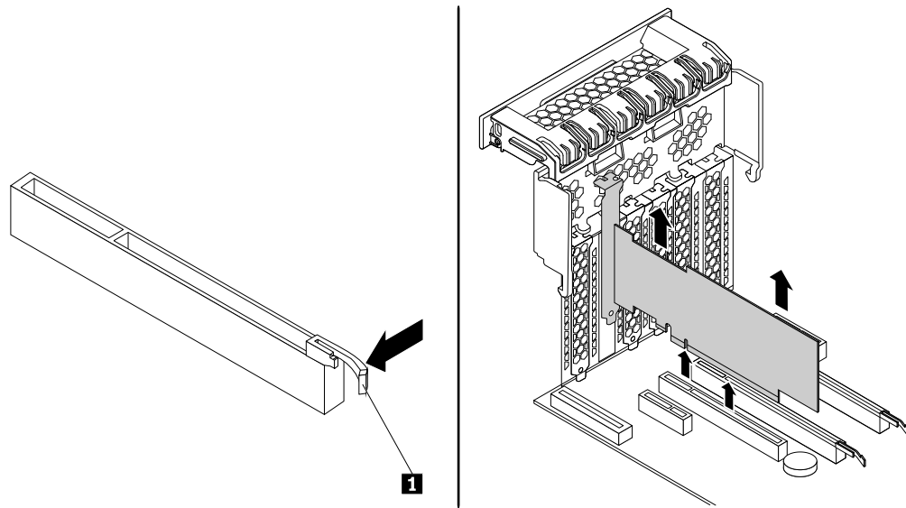
Figure 100. Removing a PCI card
