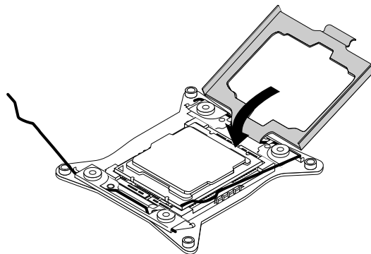
Figure 127. Closing the microprocessor retainer
