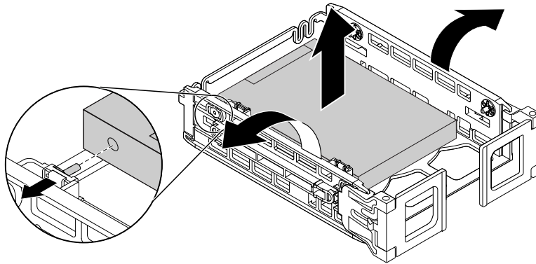
Figure 83. Removing the storage drive from the bracket
