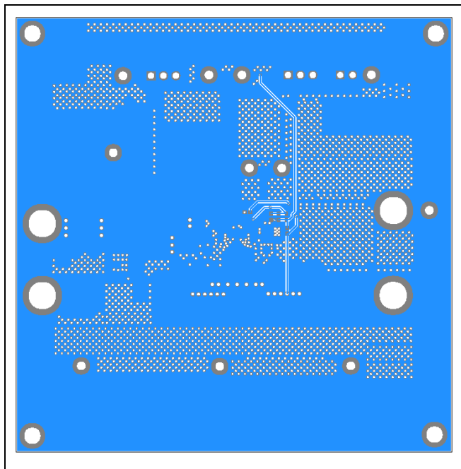
MAX26406 EV Kit PCB Layout—Bottom
