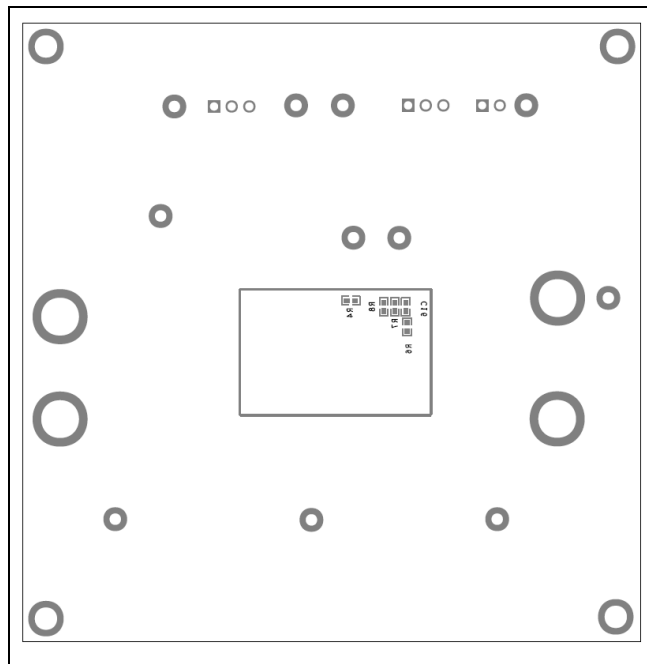
MAX26406 EV Kit Component Placement Guide—Bottom Silkscreen
