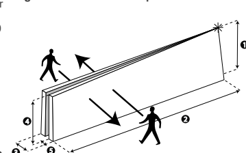
Figure 9. Detection beam pattern
