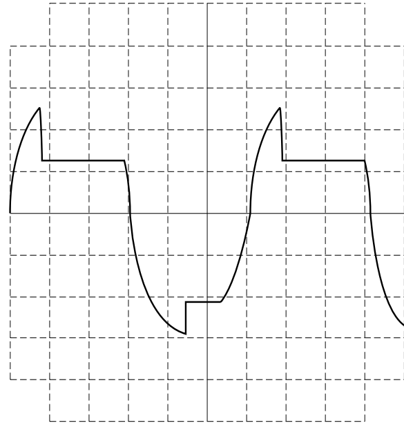
Figure 5. ODEP Limiting Wave Form
