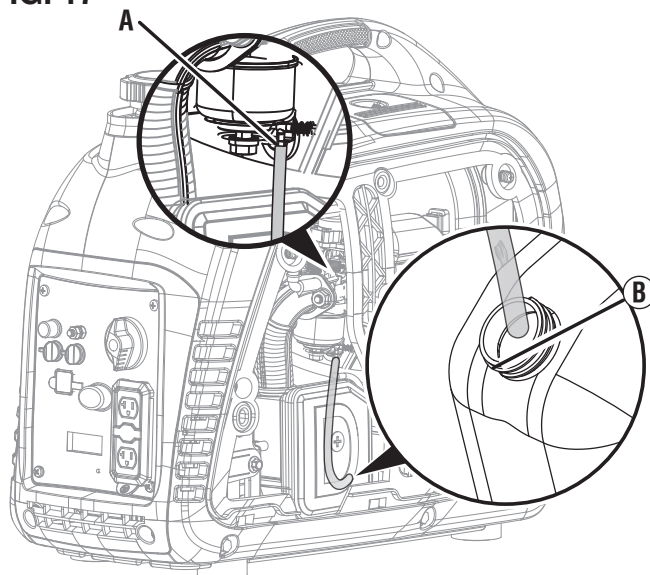
A - Valve de drainage B - Tuyau de drainage
